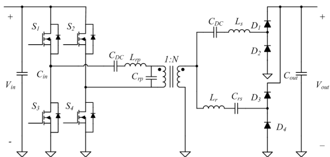
Fig. 6: Implementation of the proposed Resistance Compression Network (RCN) dc/dc converter.
