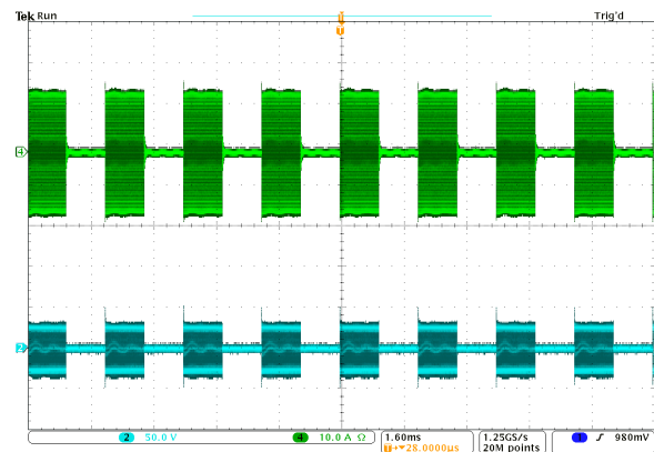
Fig. 20: (4-green) Input current and (2-turquoise) input voltage of the matching network with 50% duty ratio of on/off modulation.
