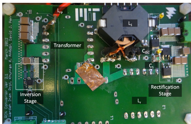
Fig. 9: Photograph of the prototype RCN dc/dc converter (Top side).
