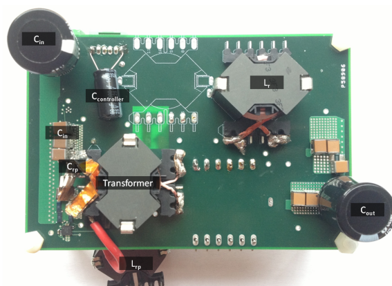
Fig. 10: Photograph of the prototype RCN dc/dc converter (Bottom side).
