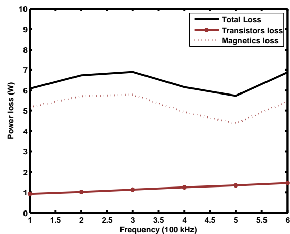
Fig. 8: Loss in the converter in the magnetics and switches when soft-switched and hard-switched at different frequencies.
