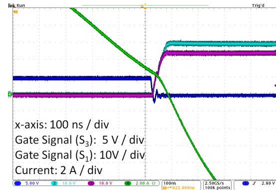
Fig. 11: Current and voltage waveforms of the RCN dc/dc converter when operated at an input voltage of 25 V: (1-blue) Gate voltage of switch S_3 , (2-turquoise) gate voltage of switch S_1 , (3-magenta) drain-source voltage of switch S_3 and (4-green) current through inductor of the matching network.
