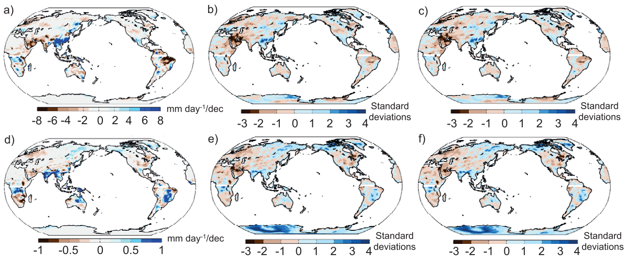
Figure 3. (a) The ensemble average summer 5-year precipitation trends ( \text{mm day}^{-1}/\text{dec} ) for the period following SRM termination in the Shutoff scenario. (b) The 5-year trends shown in (a), but normalized by the standard deviation of Historical 5-year trends at each grid point. (c) The 5-year trends shown in (a), but normalized by the standard deviation of Preindustrial 5-year trends at each grid point. ((d)–(f) are as ((a)–(c)), but for 20-year trends. The white stripe at the equator indicates the discontinuity in season from northern hemisphere to southern hemisphere (JJA and DJF, respectively). Trends over the ocean are shown in figure S6 (available at stacks.iop.org/ERL/9/024005/mmedia ).
