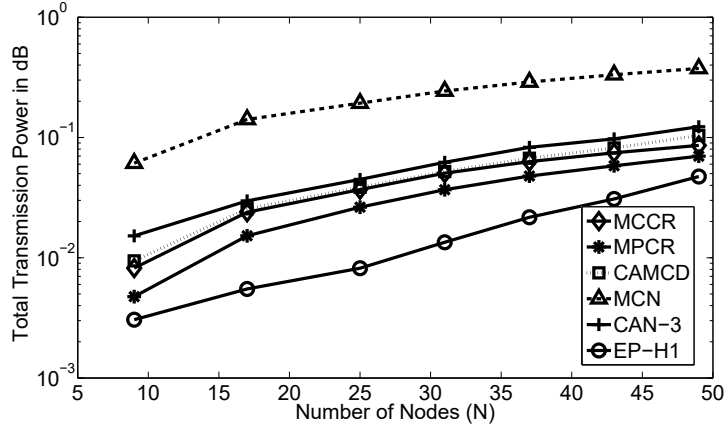
Figure 3.5: Comparing total transmission power of routing algorithms versus number of nodes ( N ) in case 2.
