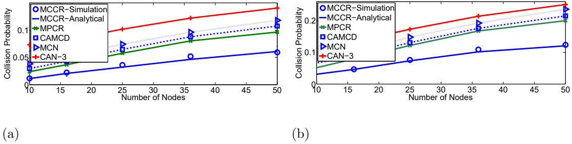
Figure 5.1: Collision Probability versus the number of relay nodes. (a) Number of flows in the network = 3 , (b) Number of flows in the network = 4.
