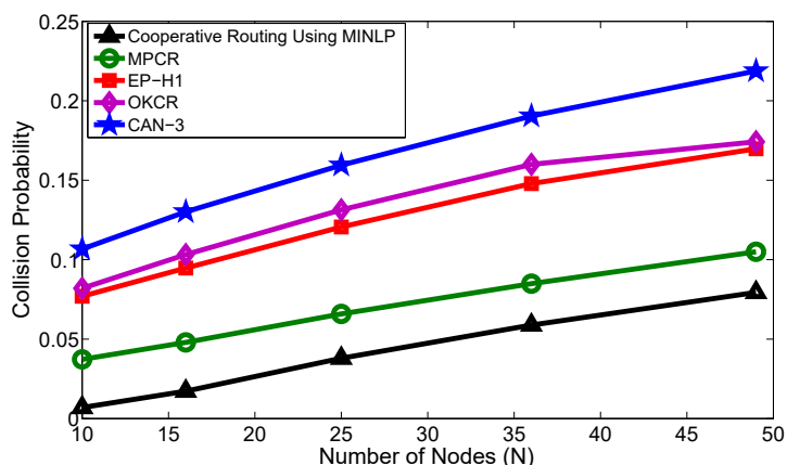
Figure 6.6: Comparing collision probability of the proposed cooperative routing and that of minimum power cooperative routing algorithms.
