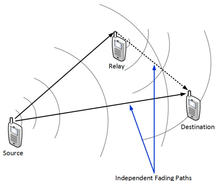
Figure 2.1: Cooperative Communication.
