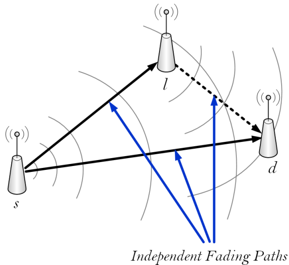
Figure 1.1: Cooperative Communication
