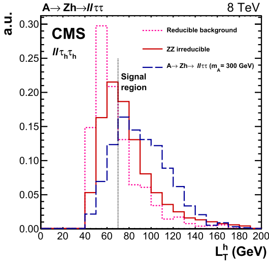
Fig. 2. Distribution of the variable L_T^h for events in the ll\tau_h\tau_h final state. The reducible background is estimated from data, instead the ZZ irreducible background from simulation.
