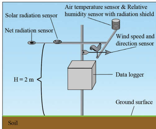
FIGURE 2. Weather station
