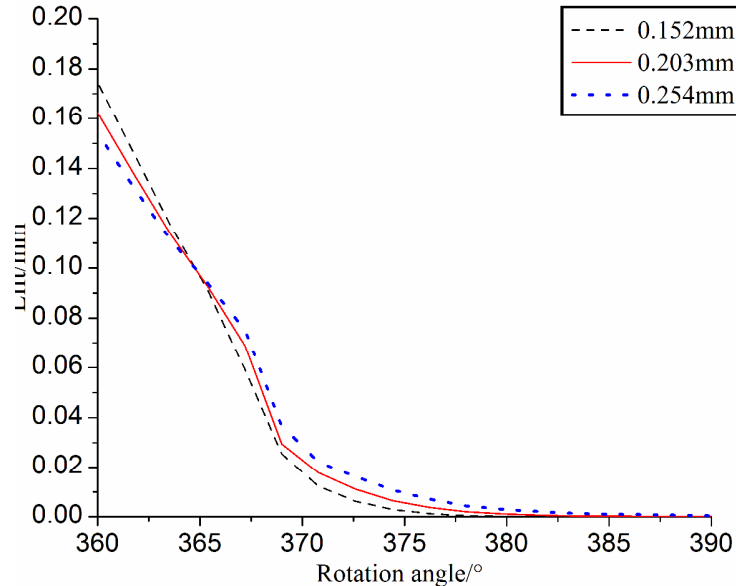
Figure 10: Enlarged figure of the lift curve at the closure point
