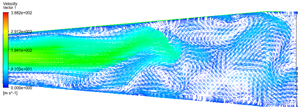
Figure 11. Velocity vectors in diffuser
