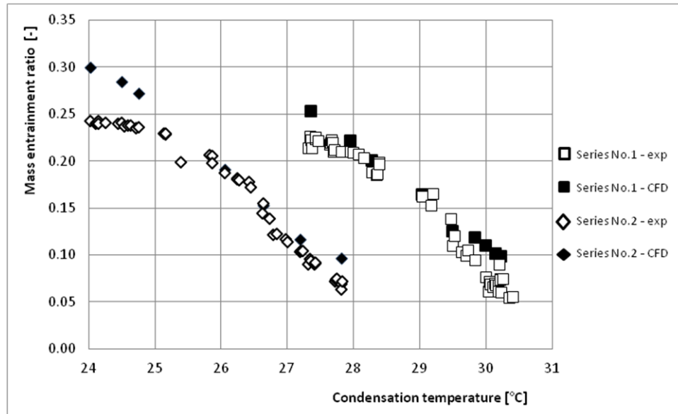
Figure 5. Performance of the tested ejector: mass entrainment ratio vs. condensation temperature
