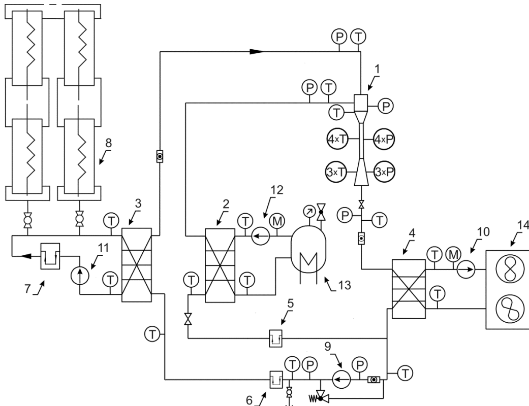
Figure 2. Schematic of testing stand: 1 – tested ejector; 2 – evaporator; 3 – vapour generator, 4 – condenser refrigerant pump; 5, 6,7 – mass flow meters; 8,13 – electric heaters; 9 – circulation pump; 10 – circulation pump in condenser cooling loop; 11 – circulation pump in evaporator heat load loop; 12 – circulation pump in evaporator heat load loop, 14 - dry cooler; T – temperature sensor; P– pressure transducers; M – mass flow meters in cooling/heating loops
