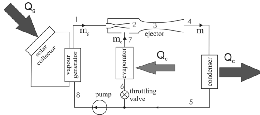
Figure. 1. Schematic of ejection refrigeration system: Q_g - motive heat, Q_e - cooling capacity, Q_c - condenser capacity, m_g - primary (motive) massflow rate, m_e - secondary (sucked in by ejector) massflow rate, m - sum of m_g and m_e , 1,2,... - thermodynamic state of working fluid
