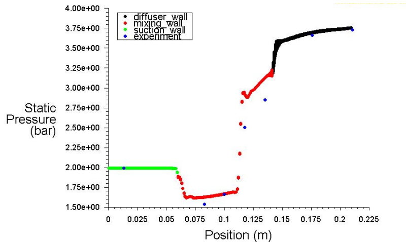
Figure 9. Pressure distribution along ejector wall for Series No. 1 (point no.1) and condensation temperature t_c = 27.3^\circ\text{C}
