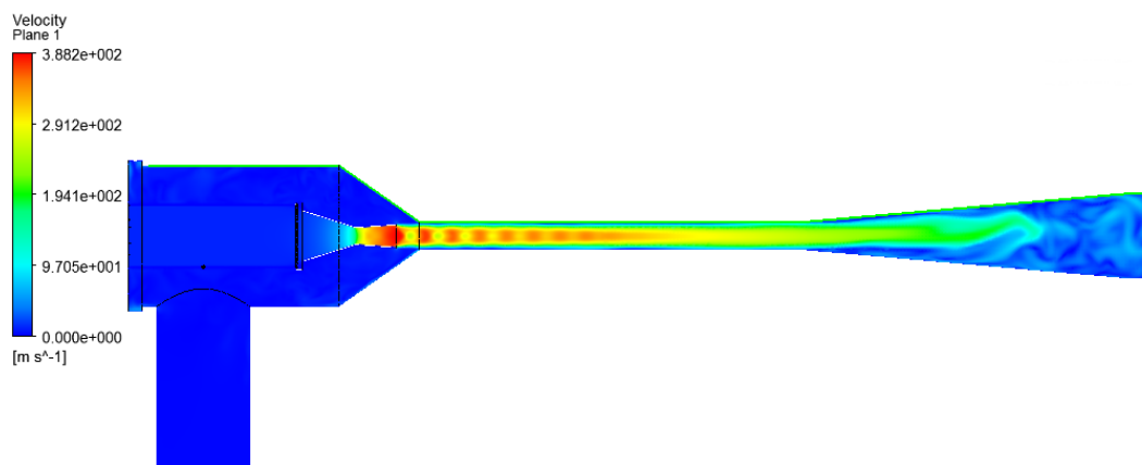
Figure 10. Velocity field in modeled ejector
