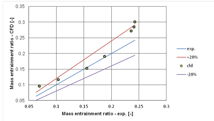
Figure 7. Deviation of the numerical results for Series No. 2
