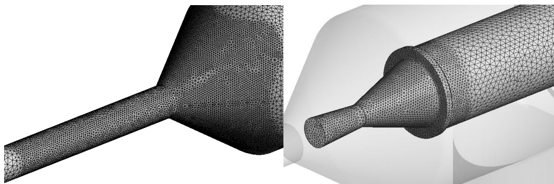
Figure 4. Part of numerical model with mesh: suction and mixing chambers (left); motive nozzle (right)
