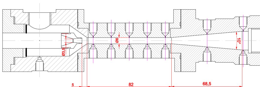
Figure 3. Schematic of tested ejector; unit: mm
