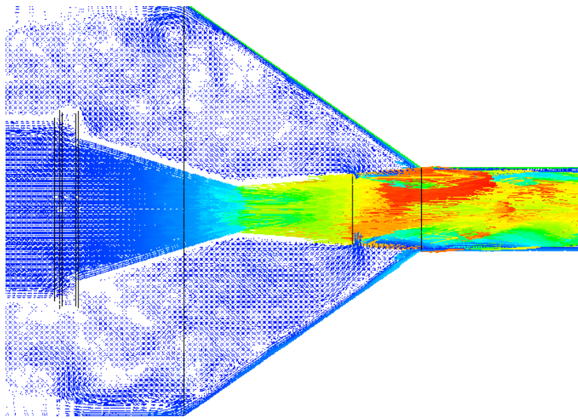
Figure 12. Velocity vectors in nozzle, suction and mixing chambers
