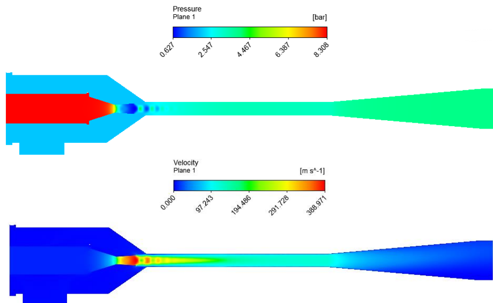
Figure 8. Pressure (top) and velocity (bottom) filed in tested ejector for Series No. 1 and condensation temperature t_c = 30^\circ\text{C}
