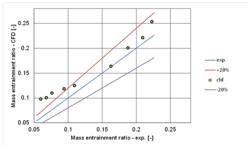
Figure 6. Deviation of the numerical results for Series No. 1
