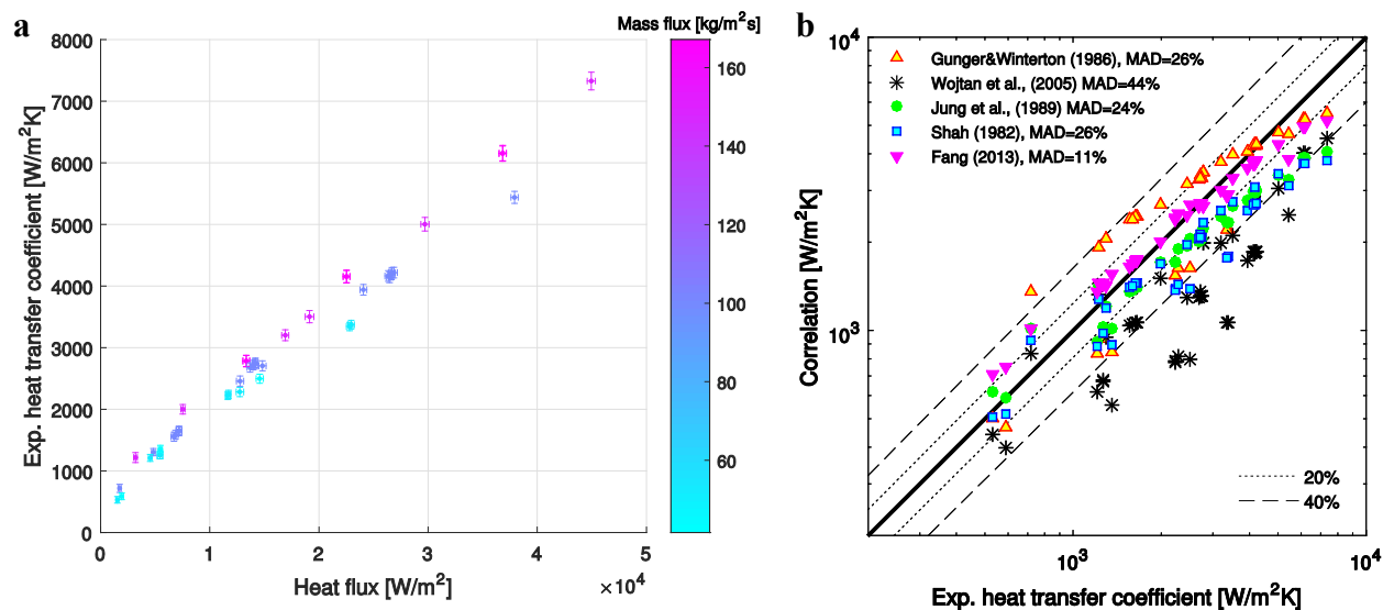
Figure 3: Experimental heat transfer coefficients vs. heat flux (a) and vs. predictions from correlations (b) for the continuous flow experiments
