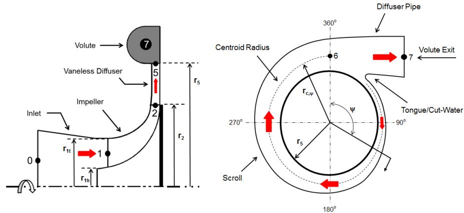
Figure 2: The centrifugal compressor stage and volute with station numbers and main dimensions
