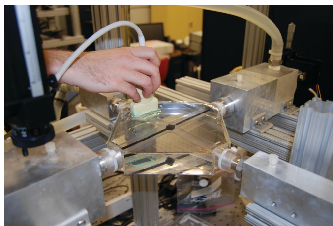
In vitro ultrasound imaging experimental setup.
