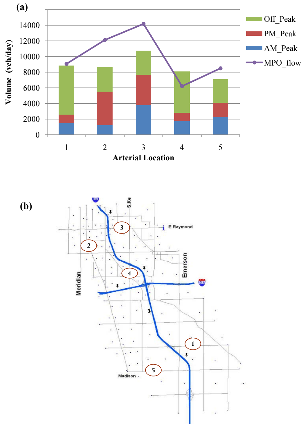
Figure 3.7 Validation of subarea analysis using traffic flow volumes on arterial links
