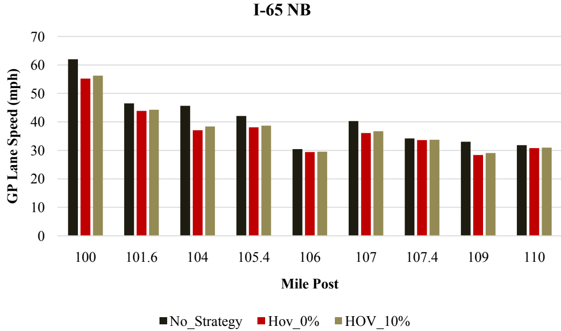
Figure 5.6 Comparison of average GP lane speed for different scenarios in NB direction of I-65
