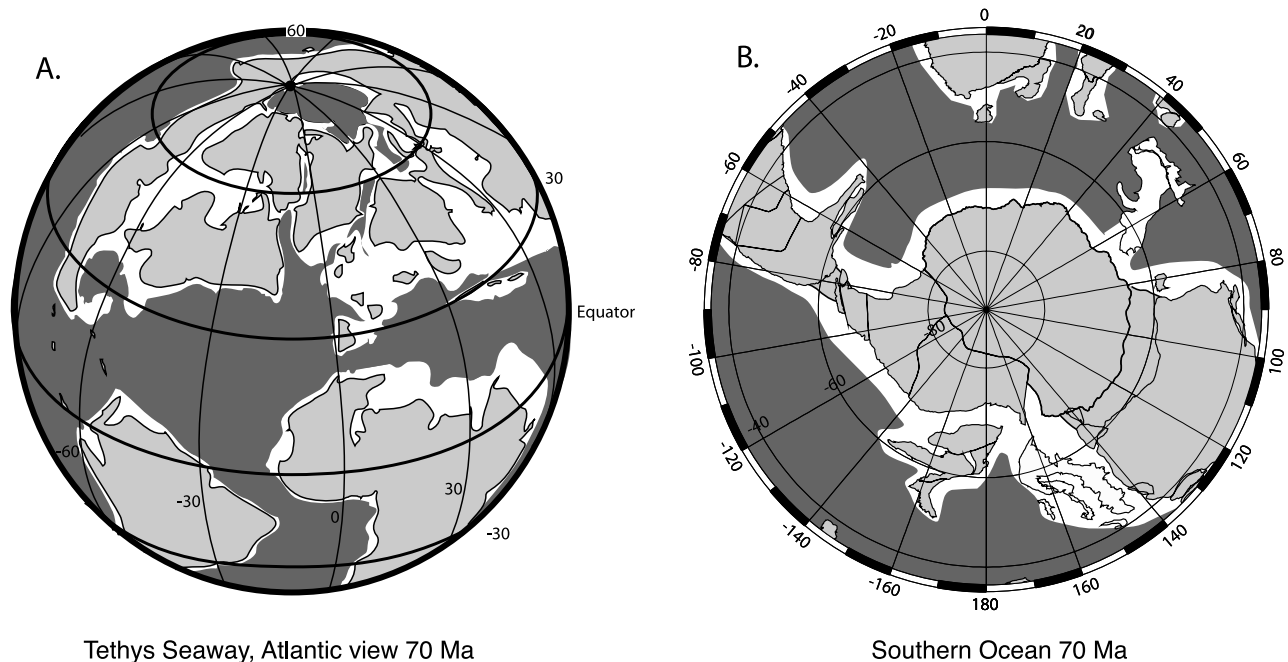
Tethys Seaway, Atlantic view 70 Ma
