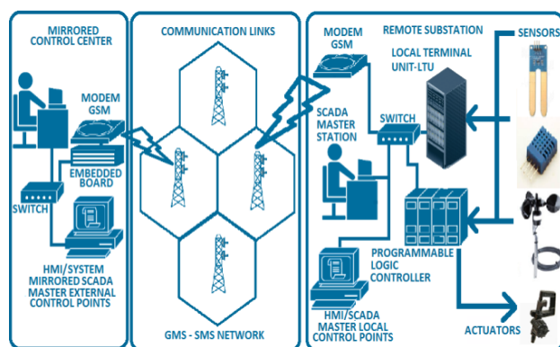
Figure 2. Proposed mirrored SCADA system.
