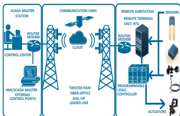
Figure 1. Typical SCADA system.
