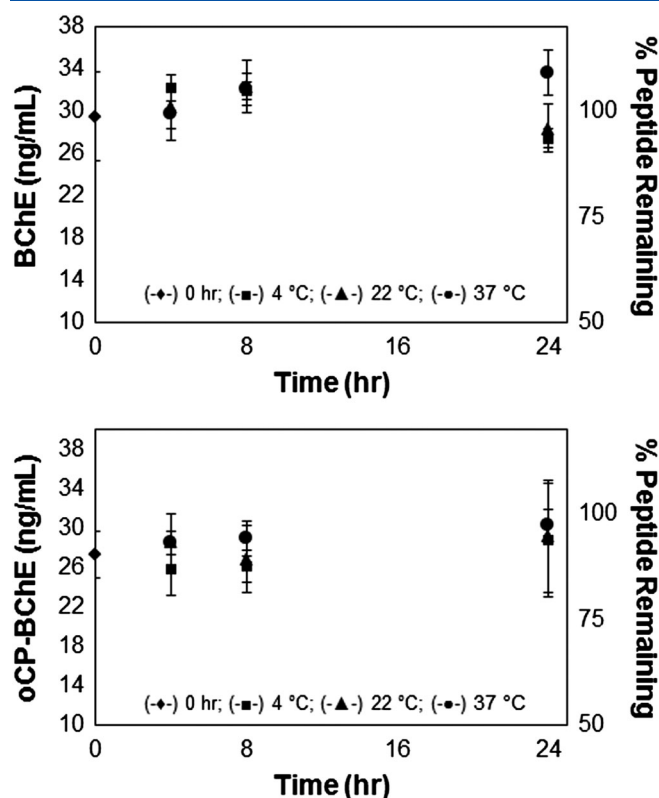
Figure 3. Stability of BChE and oCP-BChE peptide calibration standards in 0.1% formic acid buffer at 4, 22 and 37 °C. The peptides were incubated at the desired temperature for 0, 4, 8 and 24 h. Following incubation, peptides were added to matrix blank serum just prior to pepsin digestion. The calculated BChE and oCP-BChE concentrations and % peptide remaining is plotted ( n = 4 ); error bars represent \pm SD.
