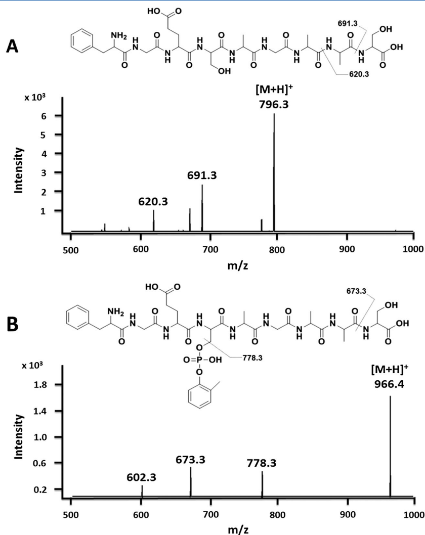
Figure 1. Chemical structures and product ion mass spectra of the precursor ions of synthetic peptides (A) BChE ( [M+H]^+ m/z 796.3); (B) oCP-BChE ( [M+H]^+ m/z 966.4). Fragmentation spectra were collected scanning the mass range of m/z 500–1000, using a collision energy of 27 V for BChE and 34 V for oCP-BChE. The dashed lines for each structure denote the proposed sites of fragmentation. The peptide sequence shown is FGESAGAAS.
