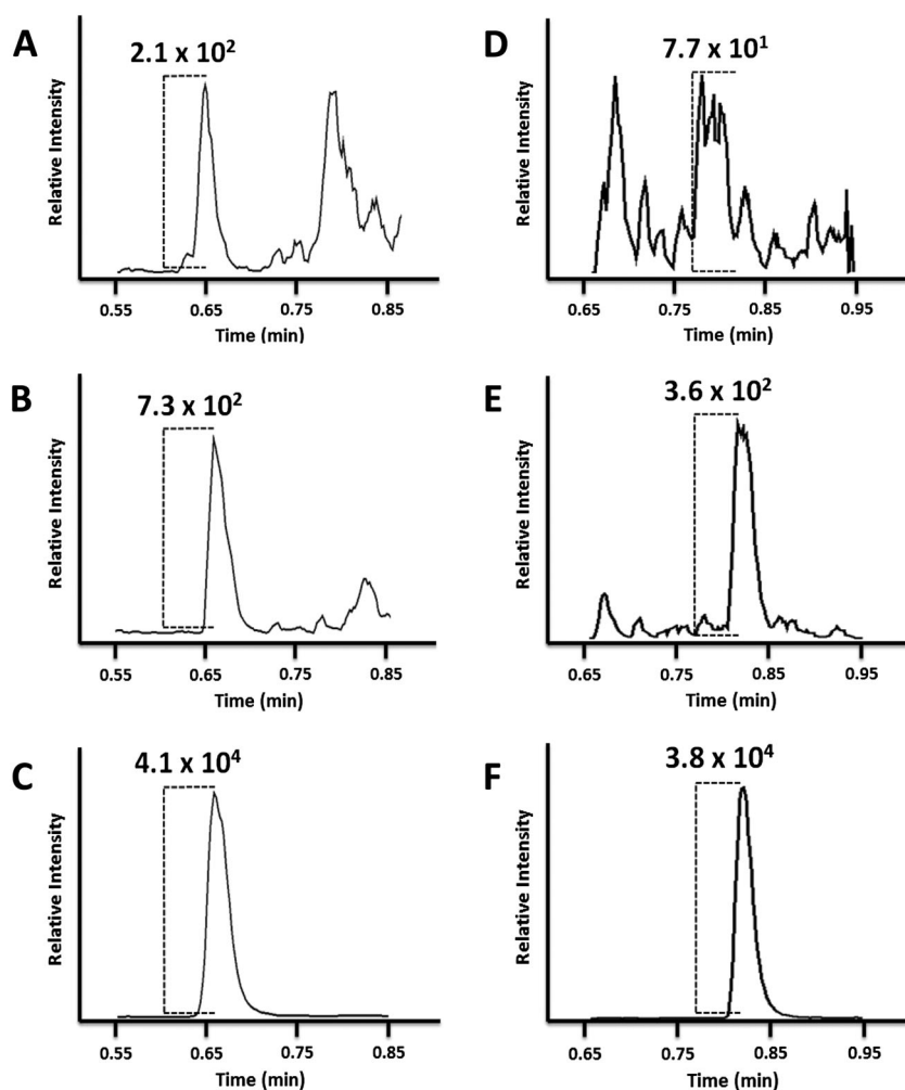
Figure 2. Extracted ion chromatograms of matrix blank serum containing (A) No synthetic BChE peptide added, peak produced from minor matrix contribution; (B) 2 ng/ml BChE (6 pg injection); (C) 150 ng/ml BChE (450 pg injection); (D) No synthetic oCP-BChE peptide added; (E) 2 ng/ml oCP-BChE (6 pg injection); (F) 150 ng/ml oCP-BChE (450 pg injection). Detection of BChE was based on the transition m/z 796.3 \rightarrow 691.3. oCP-BChE used transition m/z 966.4 \rightarrow 778.3, and quantitation was calculated from the peak area response ratio of BChE/BChE* or oCP-BChE/oCP-BChE*. The dashed lines indicate the chromatographic peak height.
