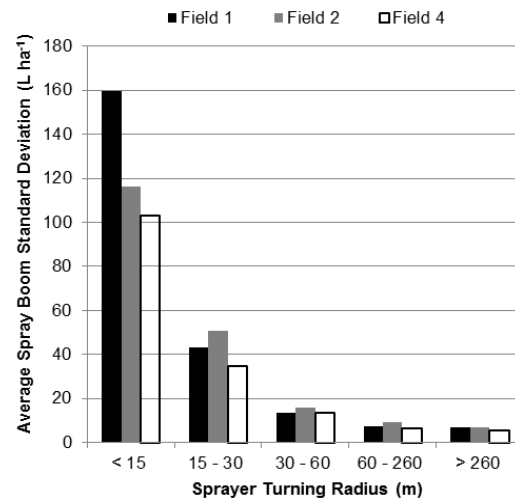
Figure 8. Average spray boom standard deviation in application rate versus selected ranges of the sprayer turning radius.
