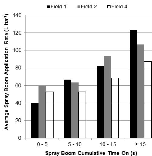
Figure 6. Average spray boom application rate versus selected ranges of cumulative time that the spray boom remained on.
