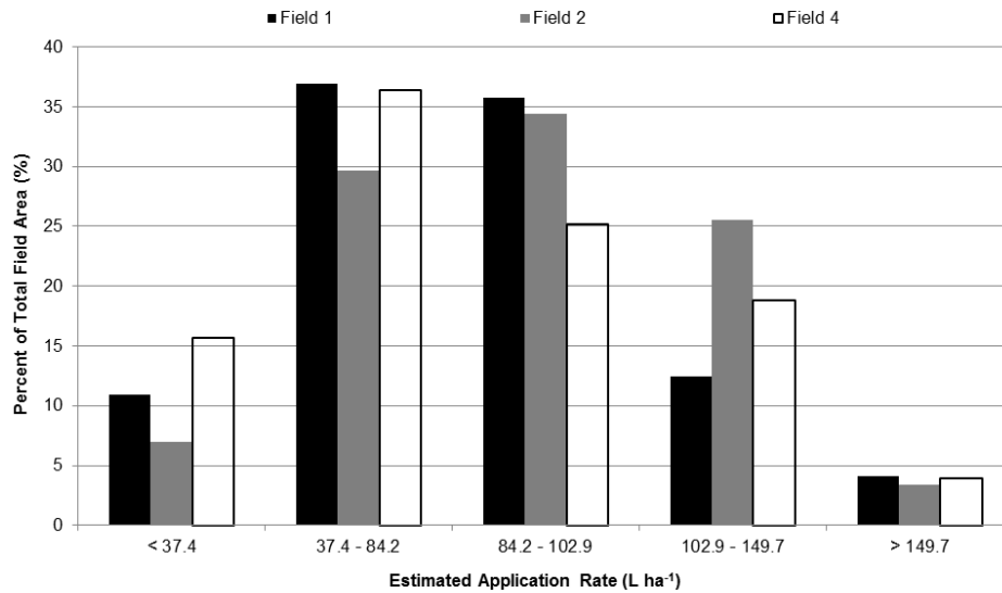
Figure 4. Distribution of field areas covered at the selected estimated application rate ranges.
