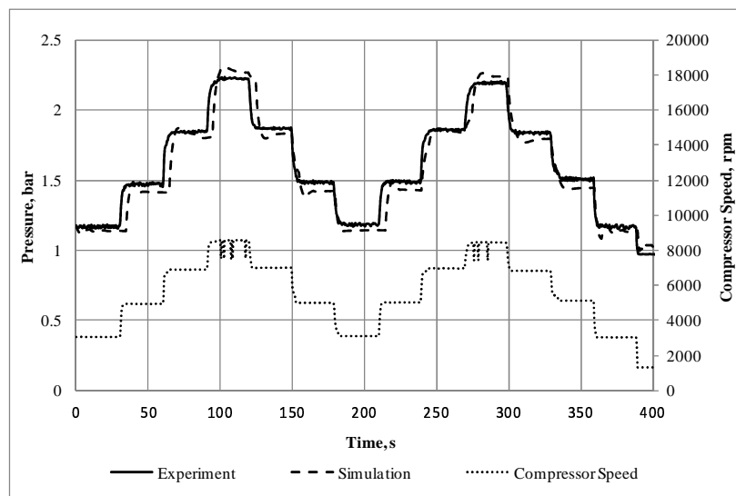
Figure 7: Comparison between experimental results and simulation data for oil-free screw compressor plant
