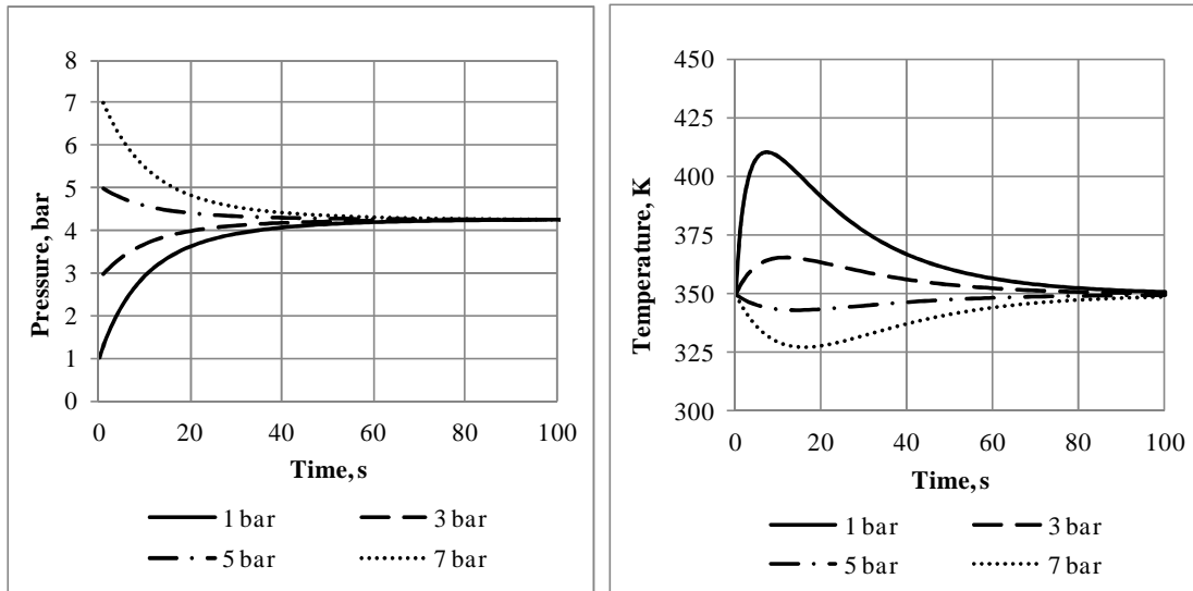
Figure 4: Pressure (left) and Temperature (right) in the tank for cases with different starting pressure in the tank
