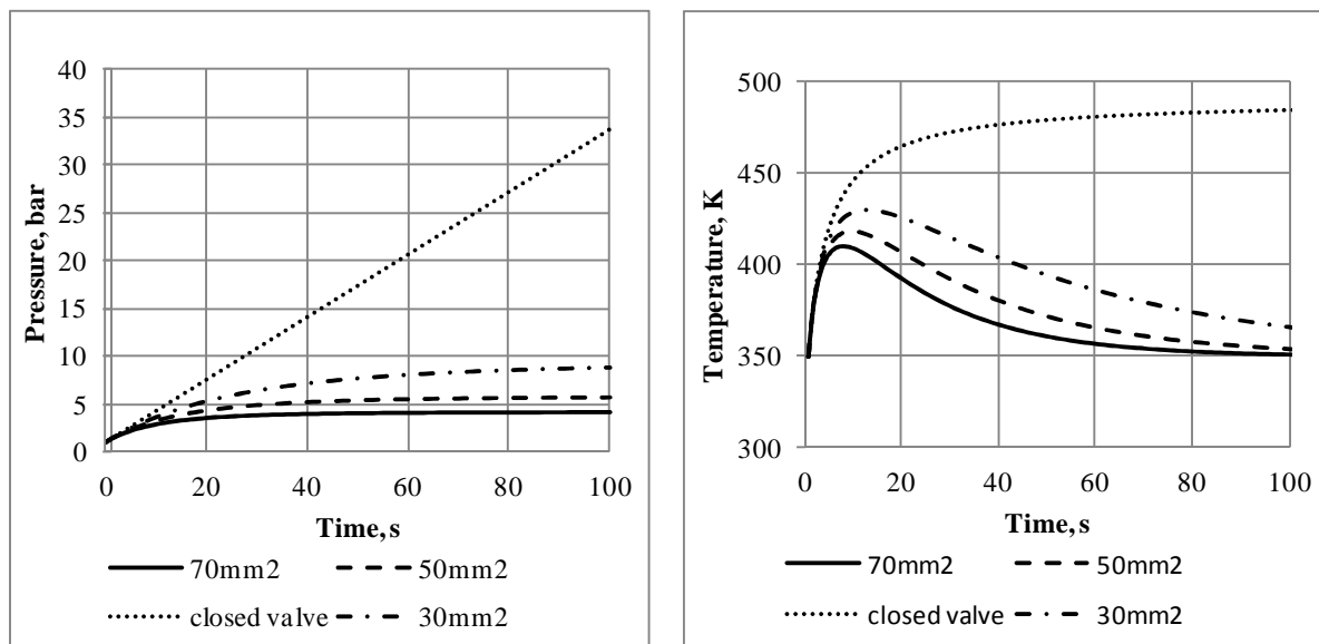
Figure 2: Pressure (left) and Temperature (right) in the tank for cases with different valve areas
