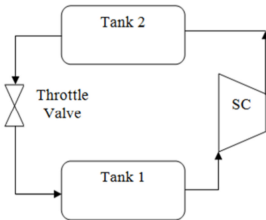
Figure 1: Scheme of Compressor Plant
