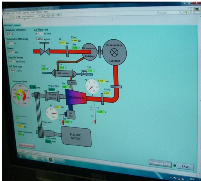
Figure 5: Test-rig Layout
