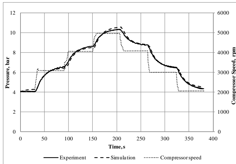
Figure 6: Comparison between experimental results and simulation data for oil-injected screw compressor plant
