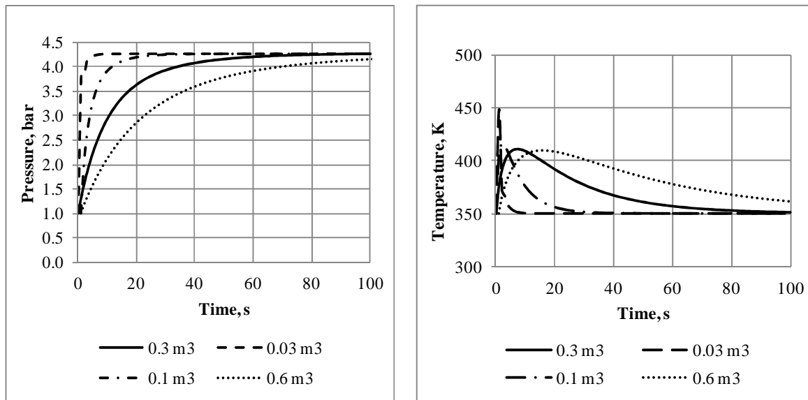
Figure 3: Pressure (left) and Temperature (right) in the tank for cases with different tank volumes
