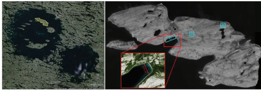
Figure 1. (left) Google Earth Landsat image of the West and East Clearwater Lakes impact features. FINESSSE field activities took place on Ile LePage, highlighted in yellow; (right) Ile LePage camp site and scale (red) and test sites (A, B, C) described in this paper (cyan).
