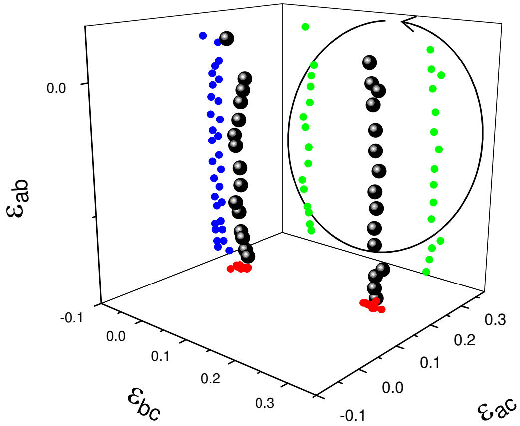
Figure 4.2: Point-by-point determined response in 3D of MO dielectric tensor components \varepsilon^{MO} from a solid flat thin permalloy film under the influence of a PL spatial hysteresis loop of field amplitude \mu_0 \mathbf{H} = 170 mT.
