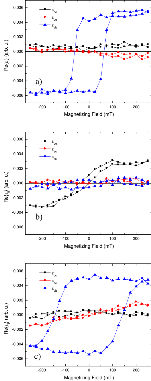
Figure 4.8: Point-by-point determined response plotted versus the magnitude of the externally applied magnetizing field of MO dielectric tensor components \epsilon^{MO} within the intrinsic coordinate system \mathbf{N}_a, \mathbf{N}_b, \mathbf{N}_c from a permalloy SCTF oriented with sample azimuth \varphi = 180^\circ film under the influence of an L, T, and P directional hysteresis scans (a), (b), and (c) respectively with maximum field amplitude of \mu_0 \mathbf{H} = 250 mT.
