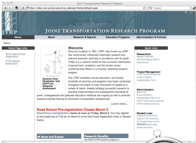
Apple Safari
