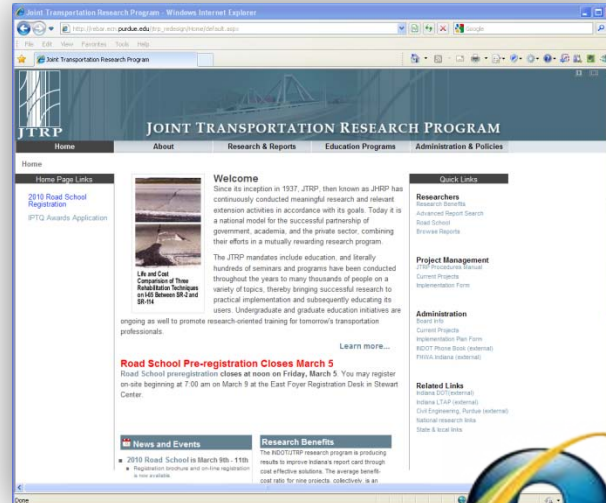
Internet Explorer 8
