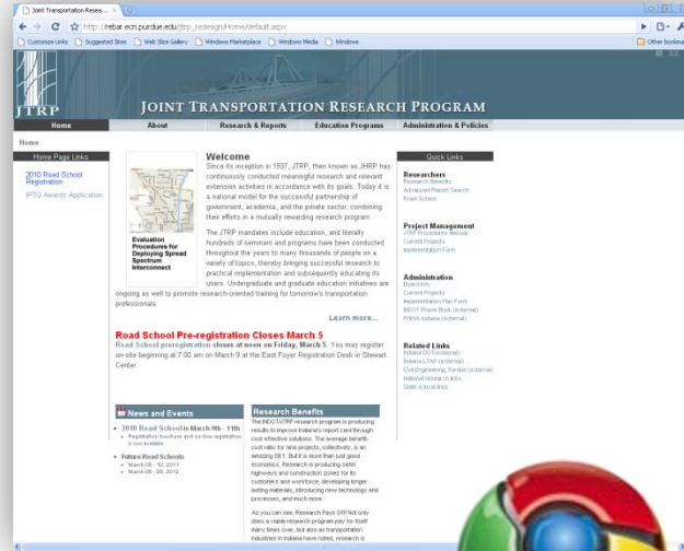
Google Chrome
