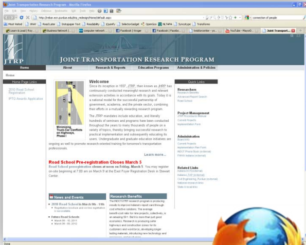
Firefox 3
