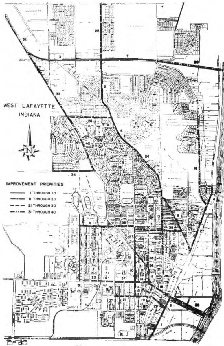
Fig. 7. Location of street sections in their order of improvement priority.
