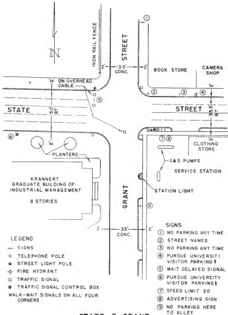
STATE & GRANT Fig. 3. Intersection diagram.
