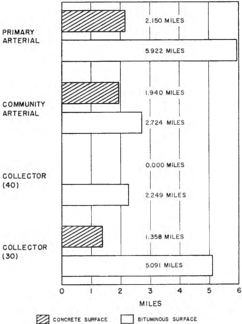
Fig. 5. Miles of street by surface type and classification.
