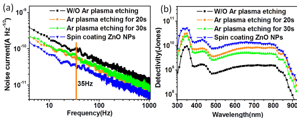
FIG. 4. For all devices at -4.5 V reverse bias. (a) The noise current curves under dark. (b) The detectivity curves.
