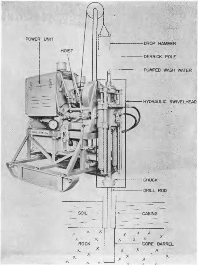
Fig. 1. Diamond core drill machine.
