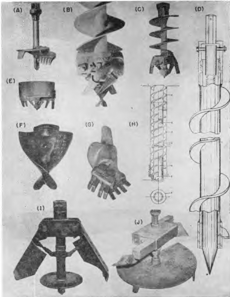
Fig. 4. Drilling and soil sampling tools for power augers.
