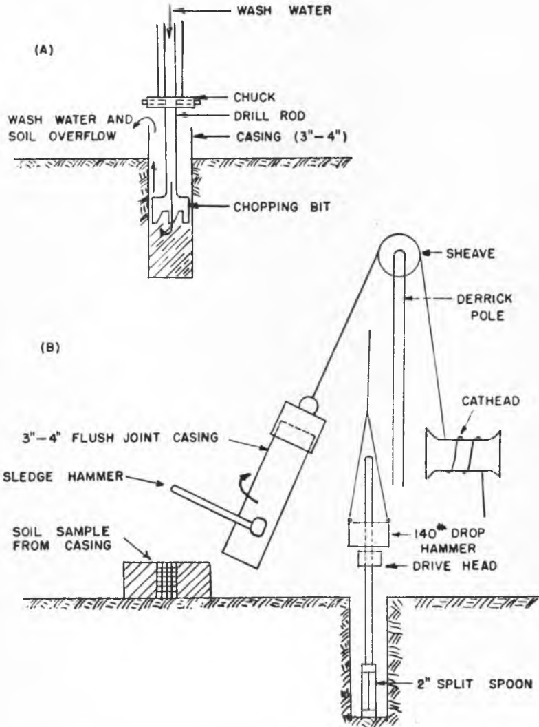
Fig. 2. Common methods of advancing and cleaning bore holes—(A) chopping and washing (B) driving casing or large spoon.
