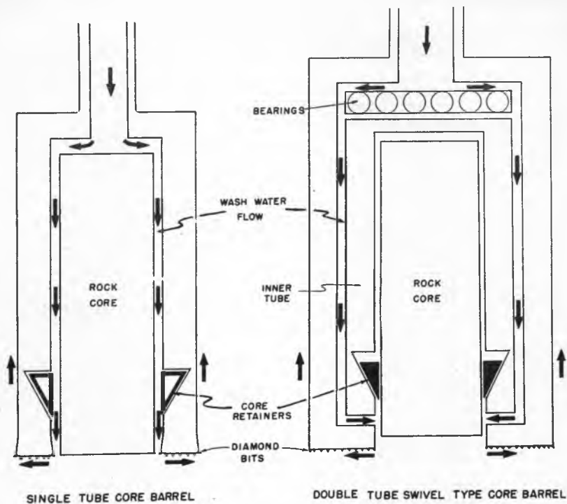
Fig. 3. Diamond bit core barrels.
