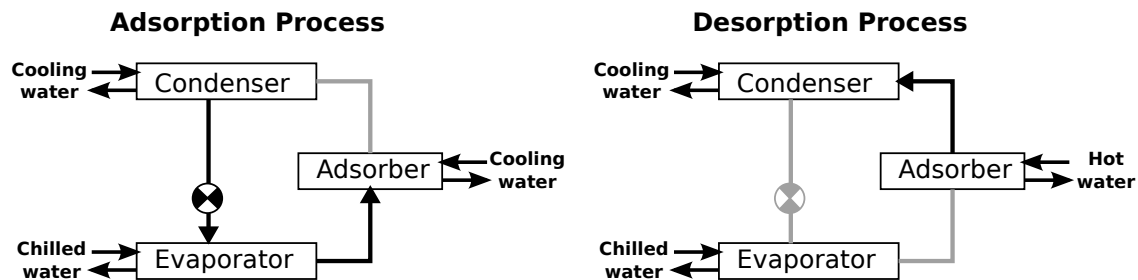
Figure 1: Schematics of one-bed adsorption cooling system
