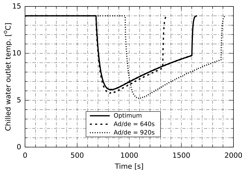
Figure 2: Comparison of chilled water outlet temperature
