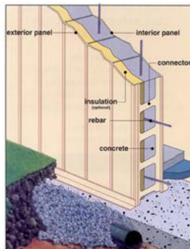
FIGURE 1 OCTAFORM: CONCEPT OF OCTAFORM (COURTESY OF OCTAFORM SYSTEM INC.)
