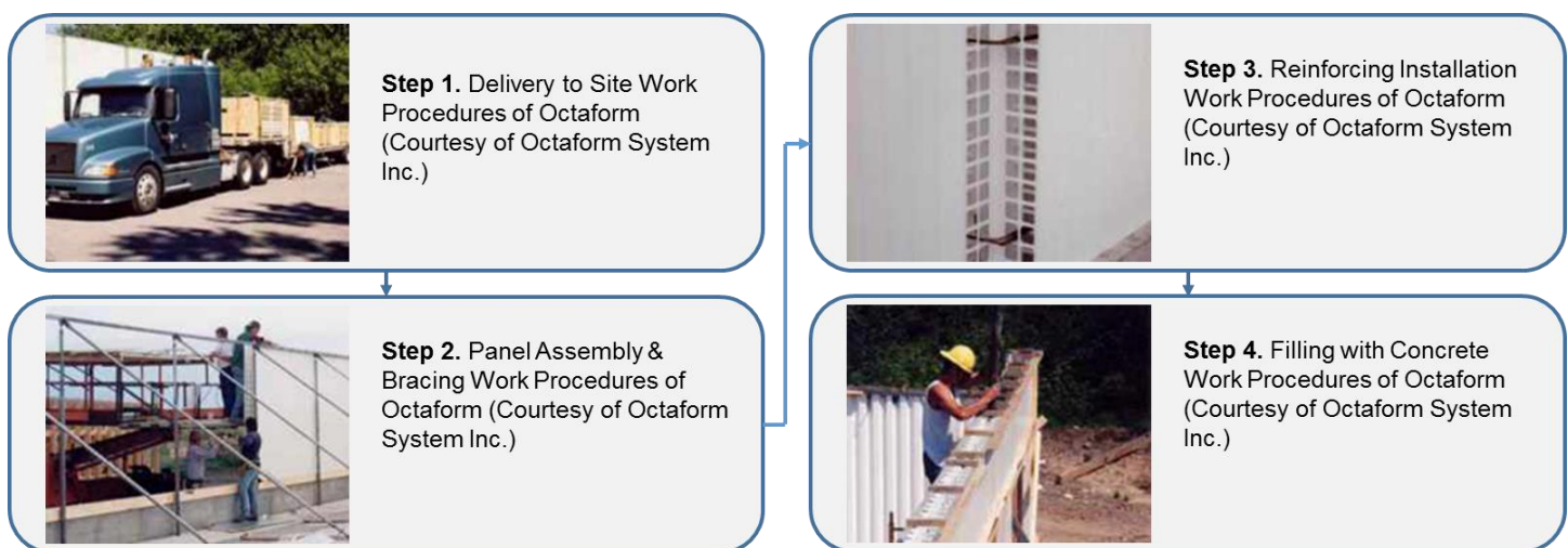
FIGURE 2 INSTALLATION PROCESS (OCTAFORM)
