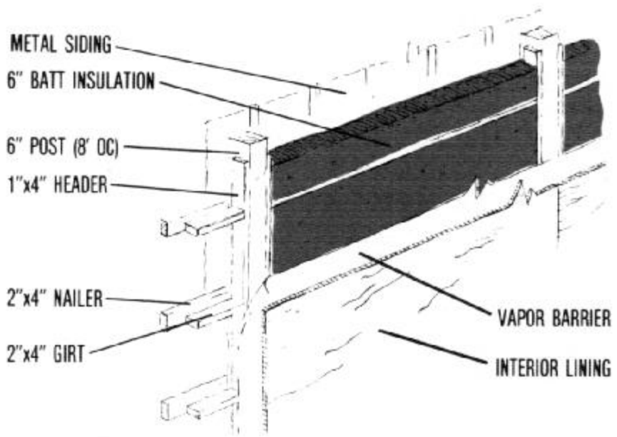
Figure 12. Post wall with 6-inch batt insulation (R=21+). Post wall with 6-inch batt insulation is beneficial in solar-heated buildings where heat conservation is especially important.
