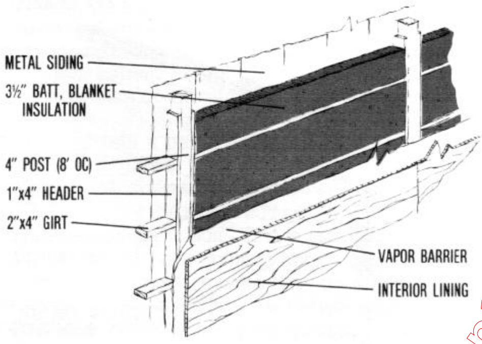
Figure 10. Post wall with batt or blanket insulation (R=13-15). This 4-inch post wall with batt or blanket insulation is common in heated buildings. It is usually more economical to build than the stud wall shown in Figure 8.
