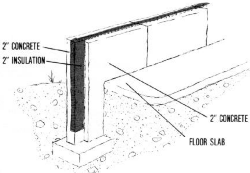
Figure 14. Pre-cast tilt-up concrete wall panels (R=11). Pre-cast tilt-up concrete wall panels may be insulated using waterproof rigid insulation. This type of wall is sometimes used for milking parlors and milk houses.
