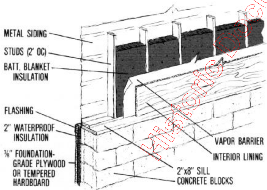
Figure 9. Concrete block and stud wall insulation (Upper wall R=13-15 if 2x4 studs, 20+ if 2x6 studs; lower wall R=12 if standard blocks, 16 if lightweight blocks with cores filled). Concrete block with stud wall above 32 inches is popular for housing large swine. Although blocks provide a 'pig-proof' wall surface next to the animals, they lose much heat and 'sweat' unless insulated.
