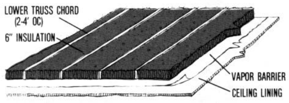
Figure 1. Loose-till, batt, blanket insulation (R=20+). Loose-till, batts and blankets are recommended as ceiling insulation in heated buildings, especially where mechanical ventilation is used.
