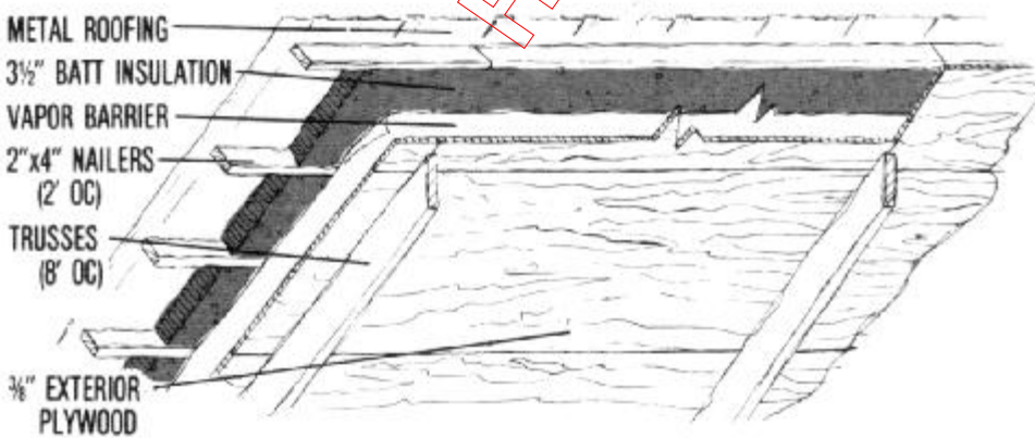
Figure 4. Insulated roof panels over trusses (R=13-15). Insulated roof panels over trusses are best fabricated on the ground and lifted into place. Roofing is then applied. This installation is recommended for modified open-front livestock housing.
