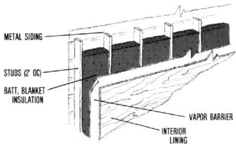
Figure 8. Stud wall insulation (R=13-15 if 2x4 studs, 20+ if 2x6 studs). Stud wall insulation is most common in heated farm buildings particular if walls are 8 feet or less in height.
