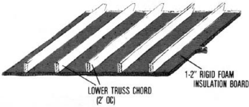
Figure 2. Ceiling with rigid insulation (R=8-16). A ceiling with rigid insulation liner is used in some shops and large animal housing. More insulation can easily be added later. Check with your insurance company about fire hazards from exposed insulation.
