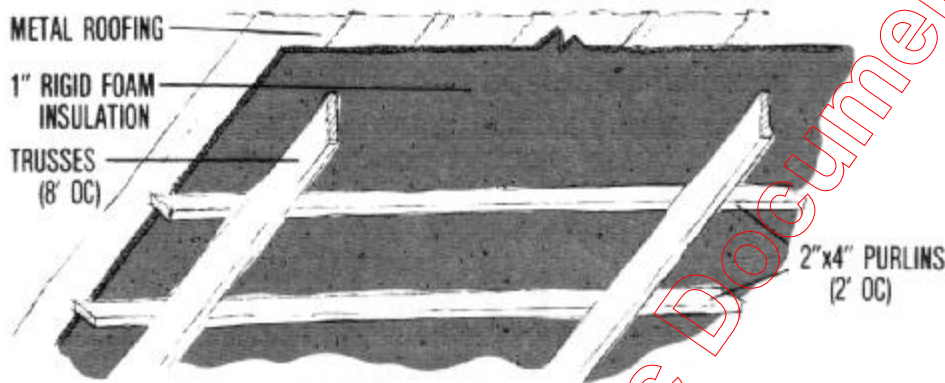
Figure 3. Rigid foam placed over purlins (R=4-9). Rigid foam placed over purlins is recommended for lightly-insulated livestock buildings and for machinery storage. The foam boards should be protected from moisture with tight-fitting tongue-and-groove joints. Screen building openings to keep birds away from the insulation. Foil faces and taped joints on top side reduce leaks.
