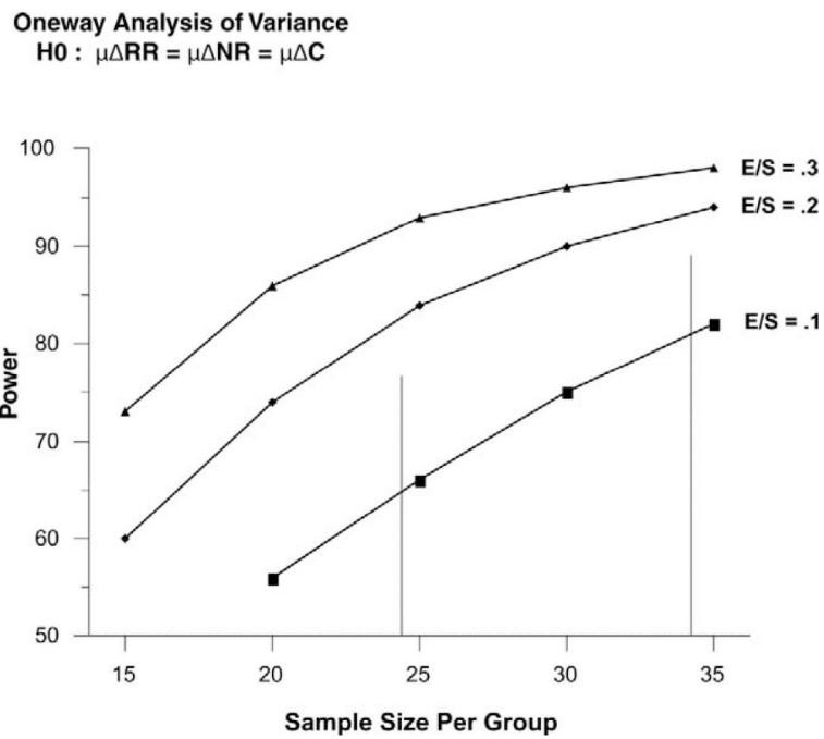
FIGURE 2. Power curves for a one-way analysis of variance with three groups and single one-way between-means contrast (comparing two of the three groups assuming the overall test is significant) generated by varying the effect size or sample size.
