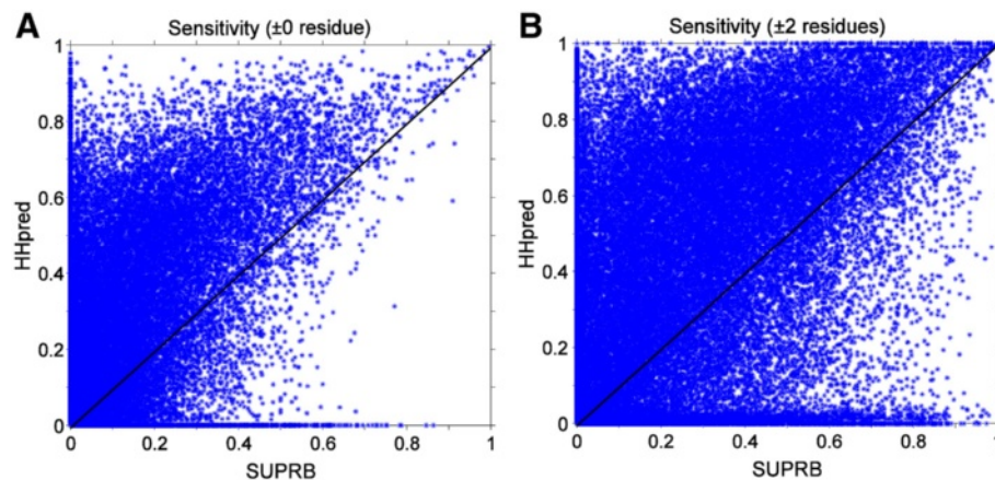
Figure 3 Comparison of the alignment sensitivity by HHpred and SUPRB. Protein pairs of the same fold were used. A , an aligned residue pair by HHpred/SUPRB is counted as correct if the pair is also aligned in the alignment by TM-align. B , an aligned pair is considered as correct if it is within two residue shift from an aligned pair in the TM-align alignment.
