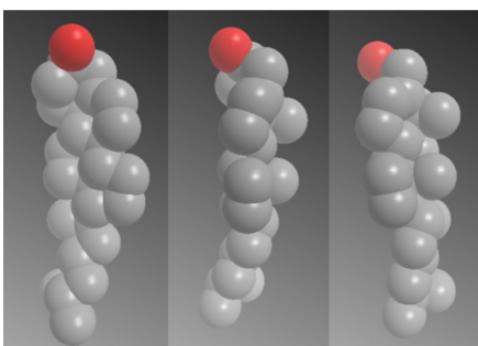
Figure 1.5 Planar nature of cholesterol structure. A space filling display of cholesterol's smooth \alpha -face, end view and rough \beta -face with protruding methyls.
