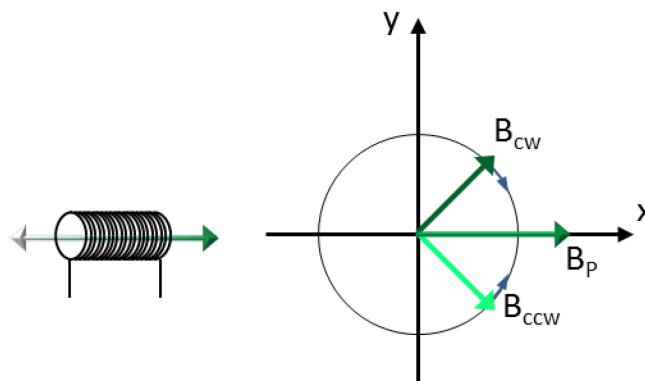
Figure 2.8 The oscillating magnetic field created along the sample coil axis taken to be the x axis in the lab frame. This field can be thought of as the sum of two field vectors rotating in phase with the same angular frequency, clockwise and counterclockwise about the z axis (viewed from above the coil).
