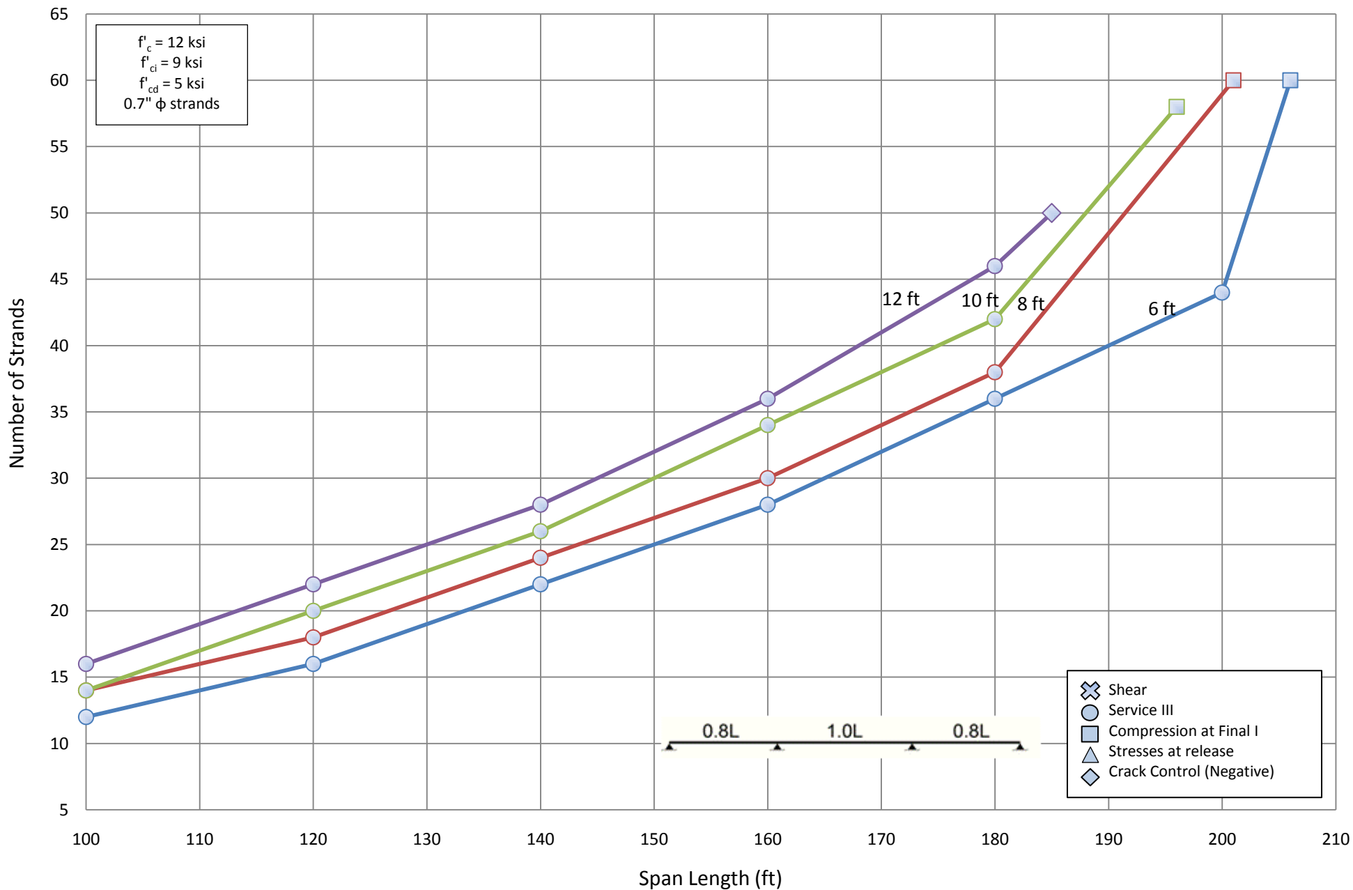
Number of Strands for NU 1350 - Three Span (1.0L)
