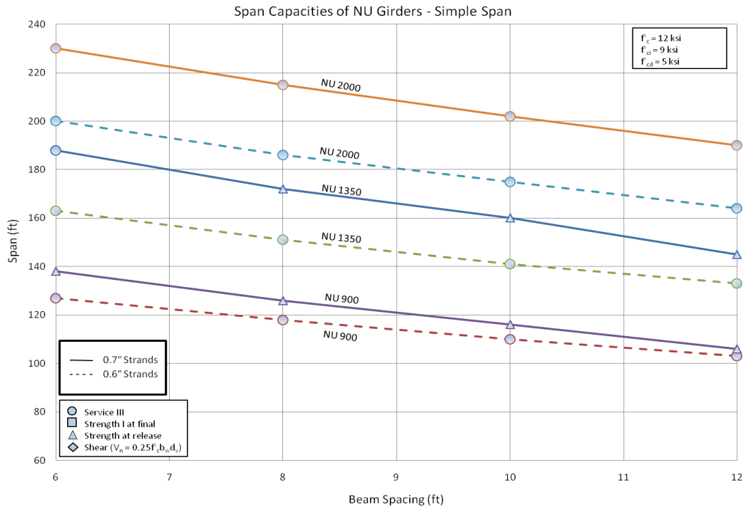
Figure 5 Summary chart comparison between 0.6 and 0.7 inch strands.
