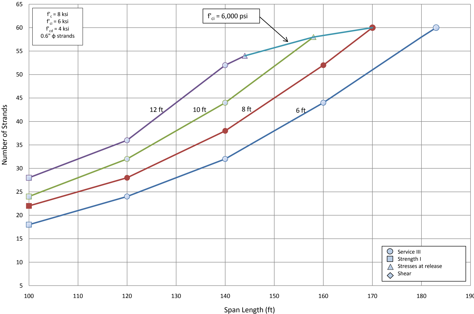
Number of Strands for NU 1800 - Simple Span
