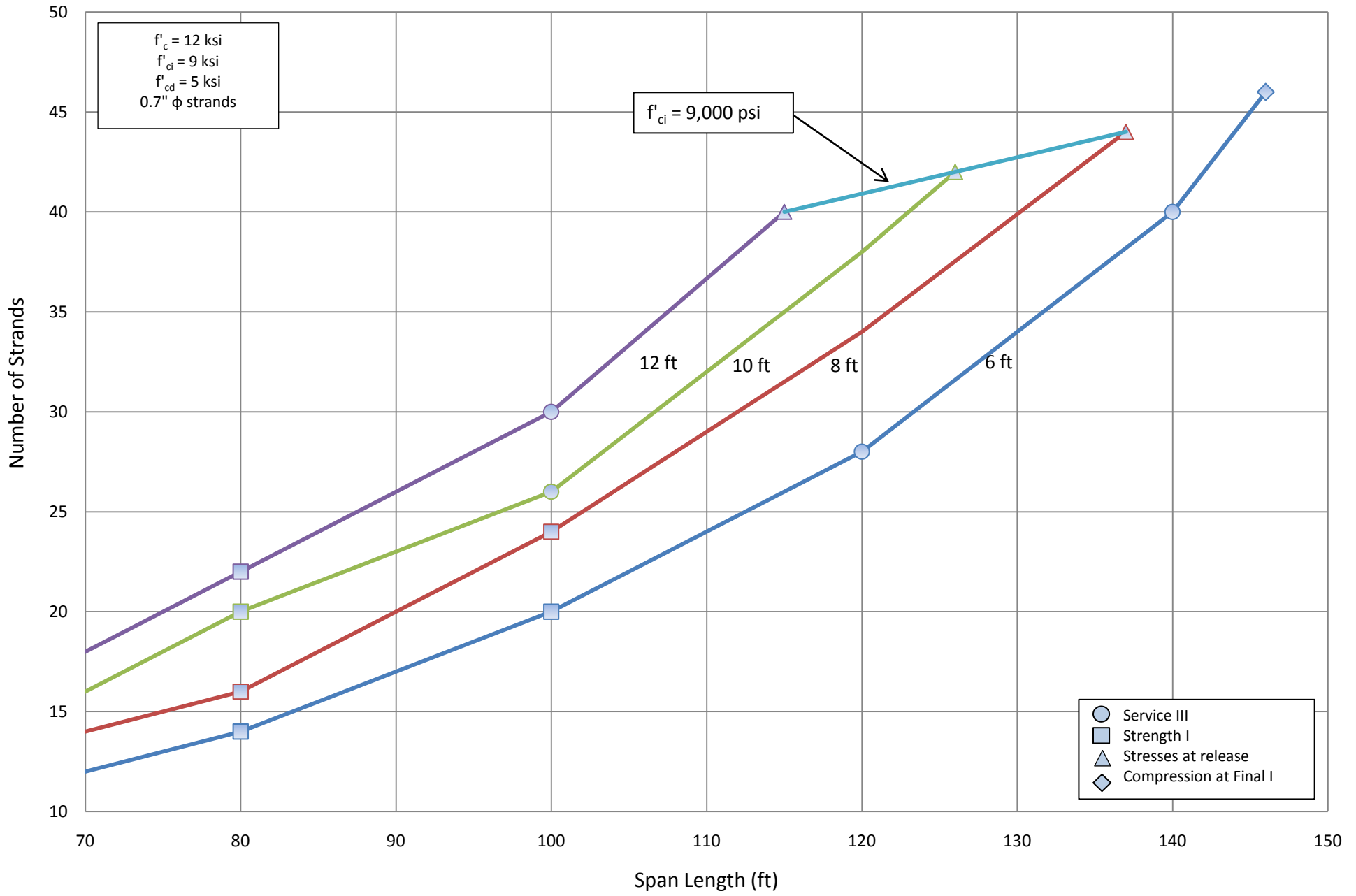
Number of Strands for NU 1100 - Simple Span
