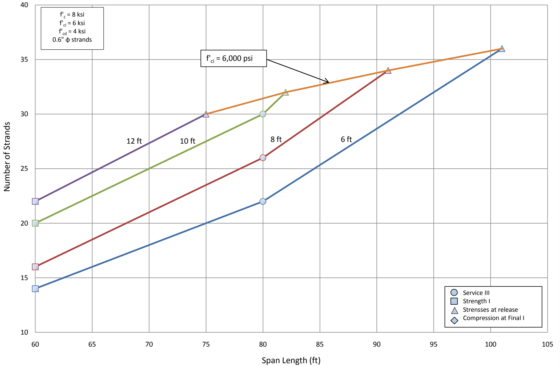
Number of Strands for NU 900 - Simple Span
