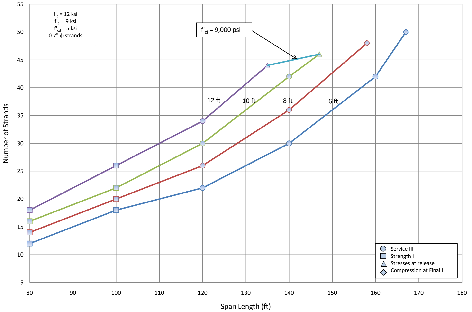
Number of Strands for NU 1350 - Simple Span
