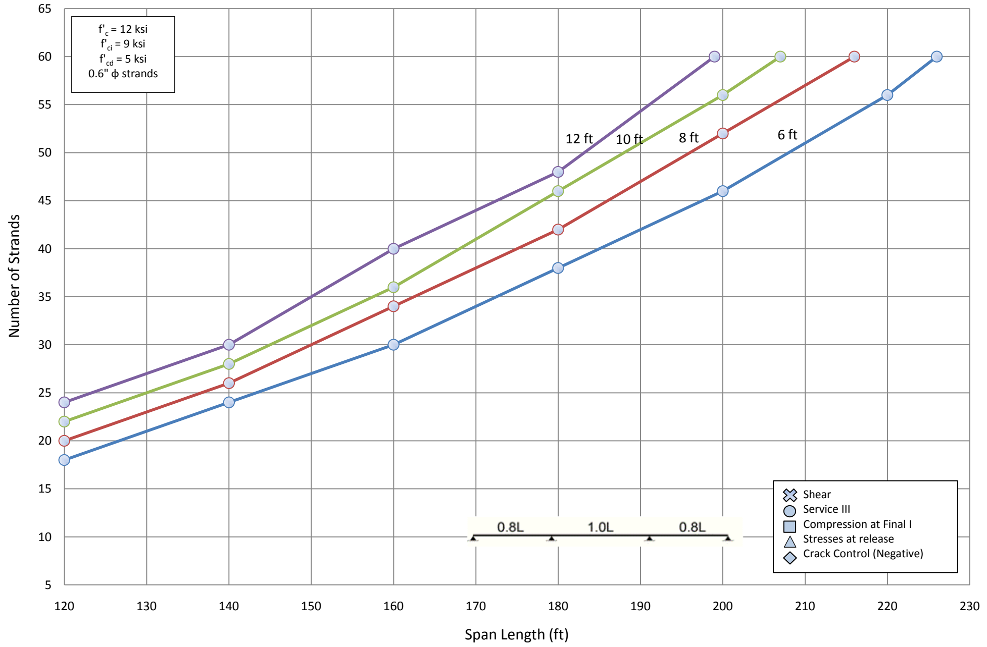
Number of Strands for NU 1800 - Three Span (1.0L)
