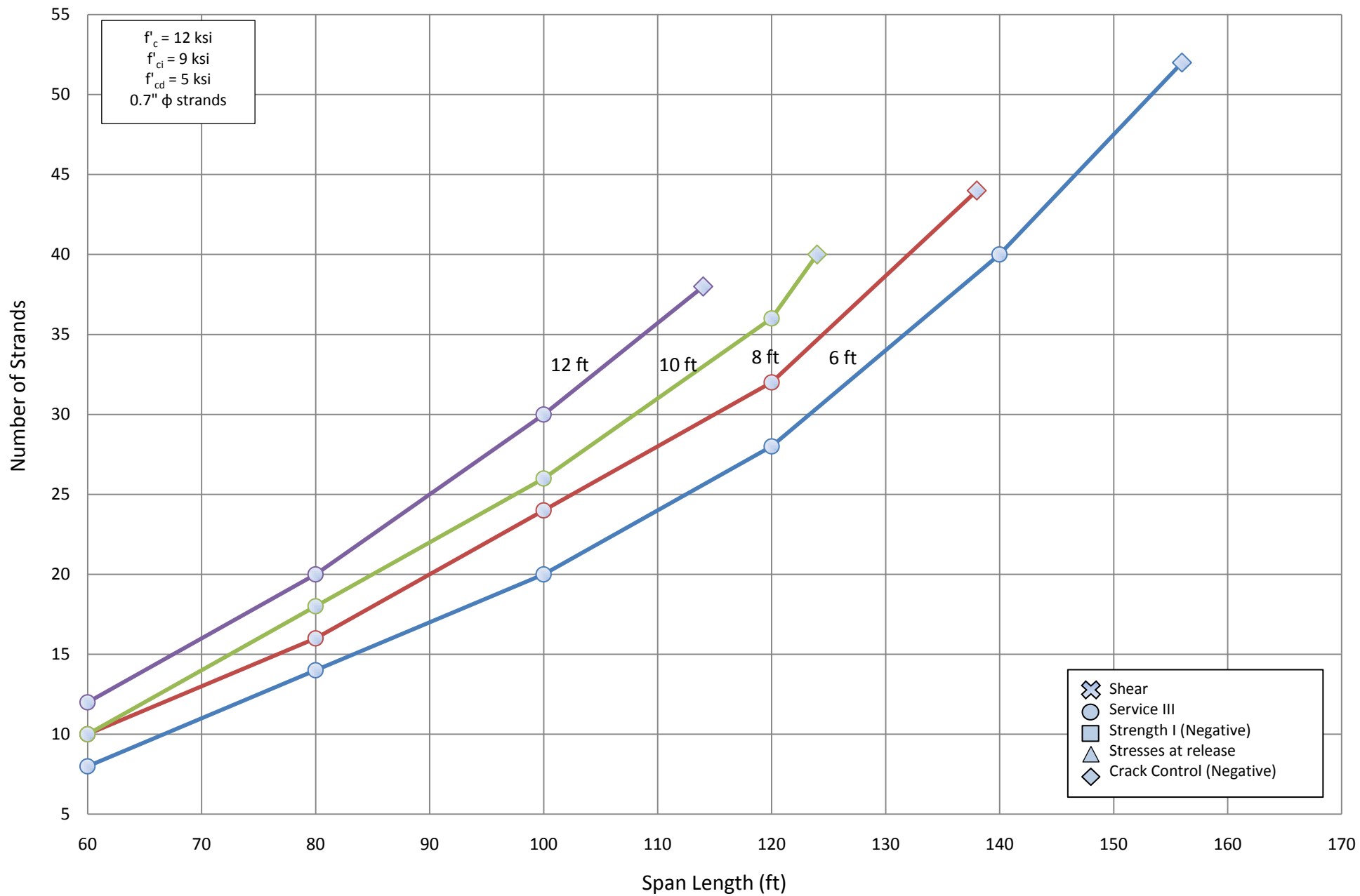
Number of Strands for NU 900 - Two Span
