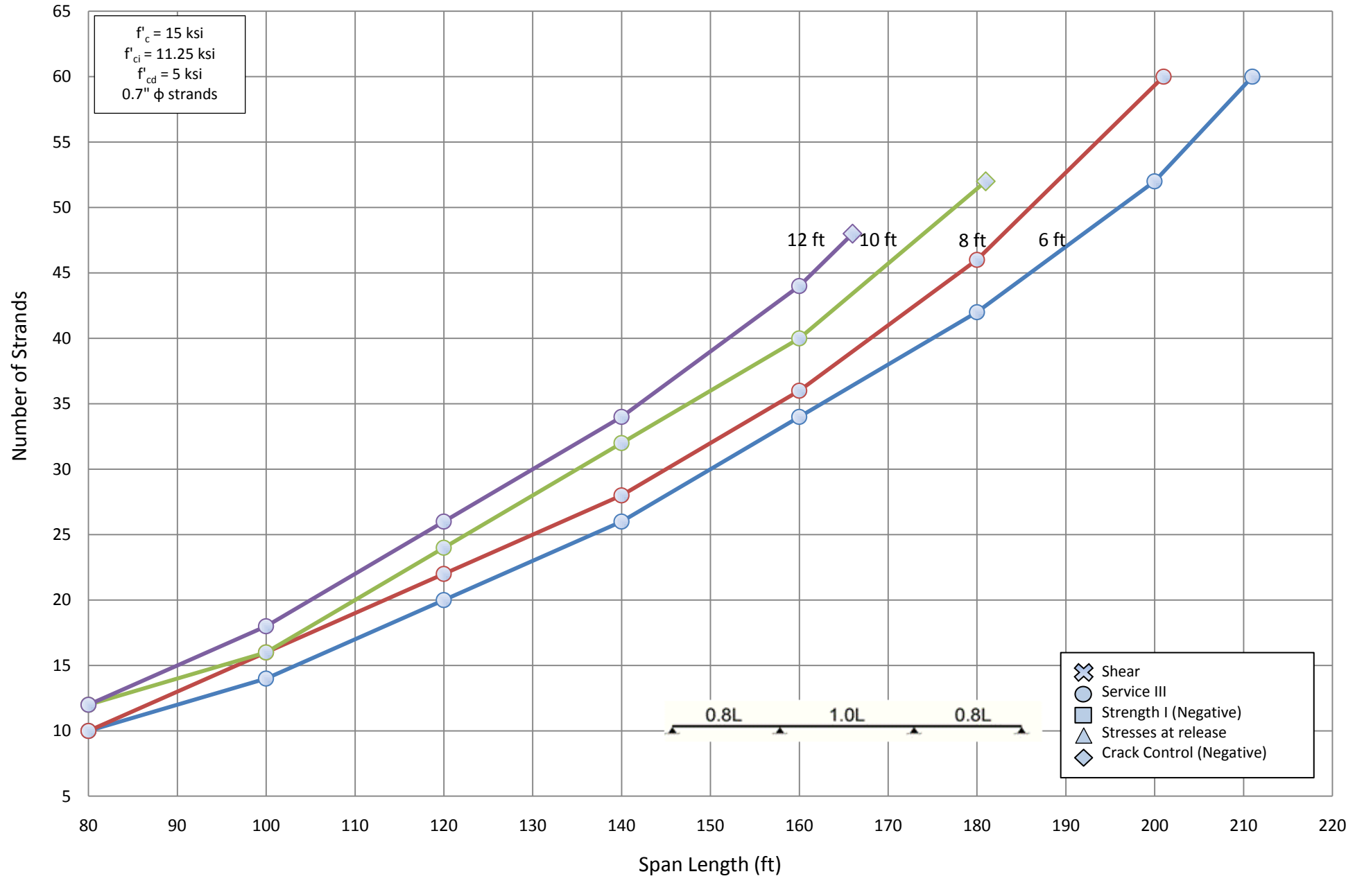
Number of Strands for NU 1100 - Three Span (1.0L)
