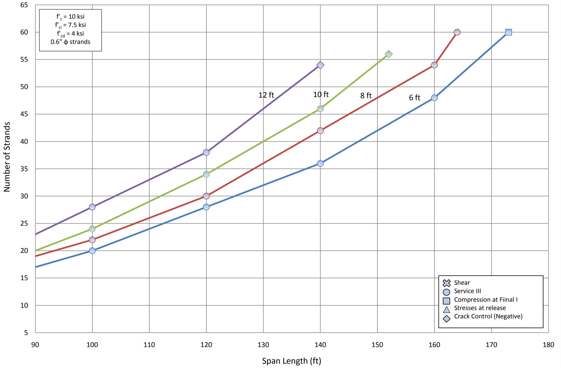
Number of Strands for NU 1350 - Two Span
