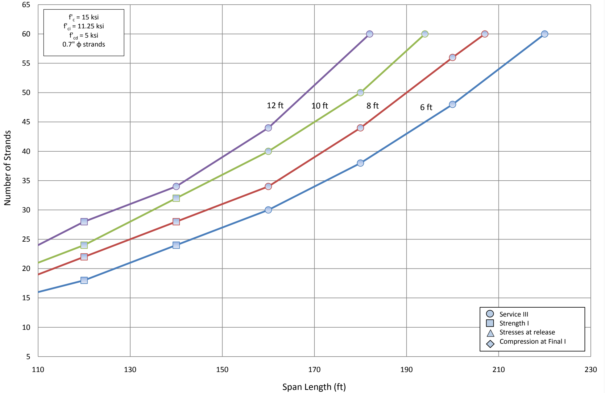
Number of Strands for NU 1800 - Simple Span
