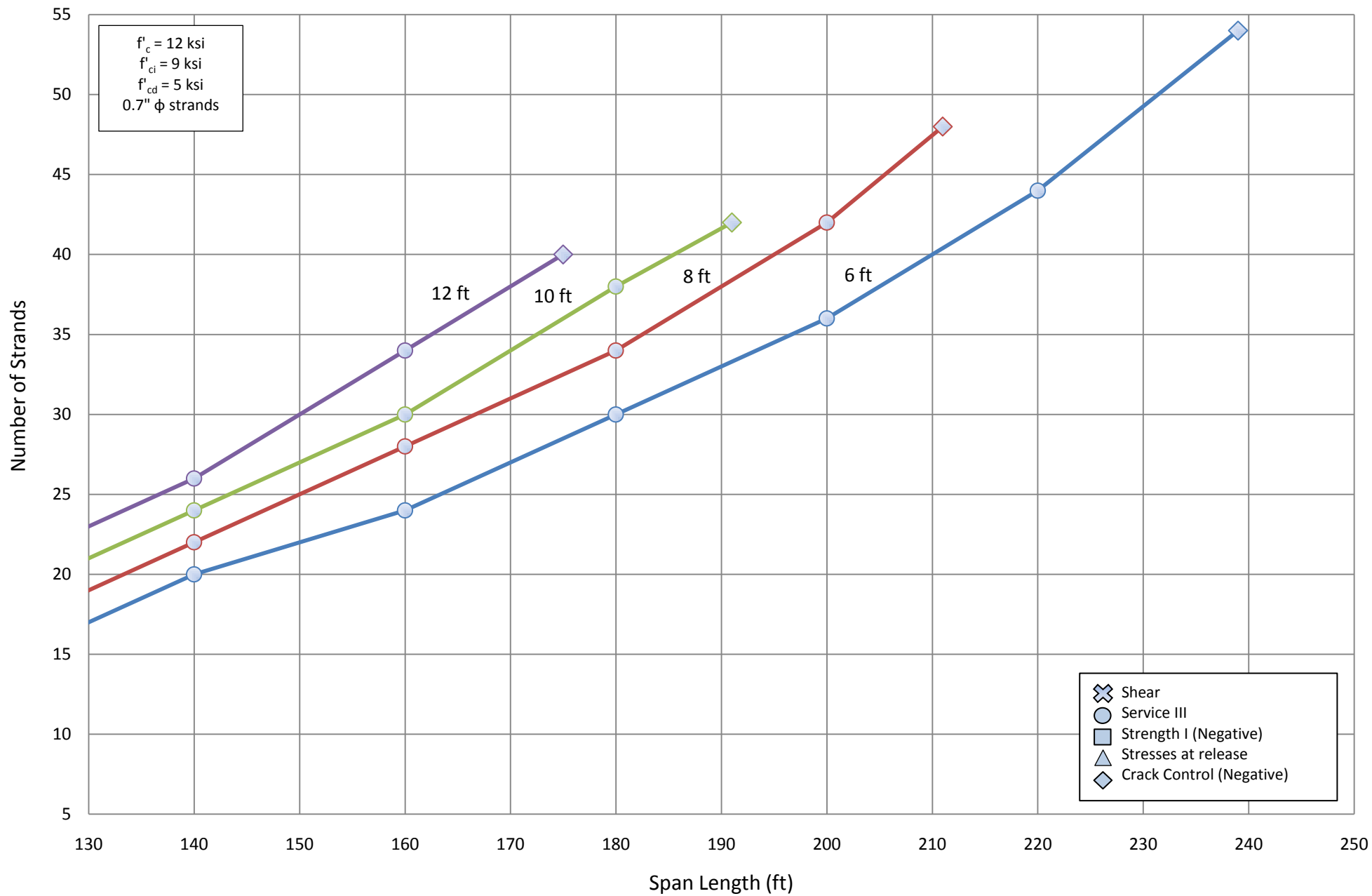
Number of Strands for NU 2000 - Two Span
