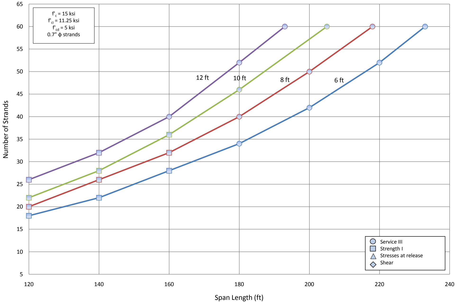
Number of Strands for NU 2000 - Simple Span
