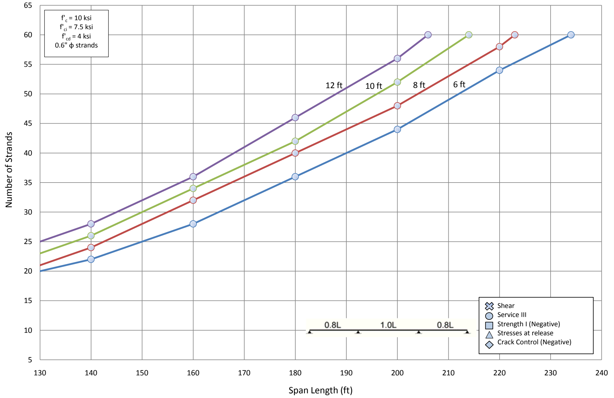
Number of Strands for NU 2000 - Three Span (1.0L)
