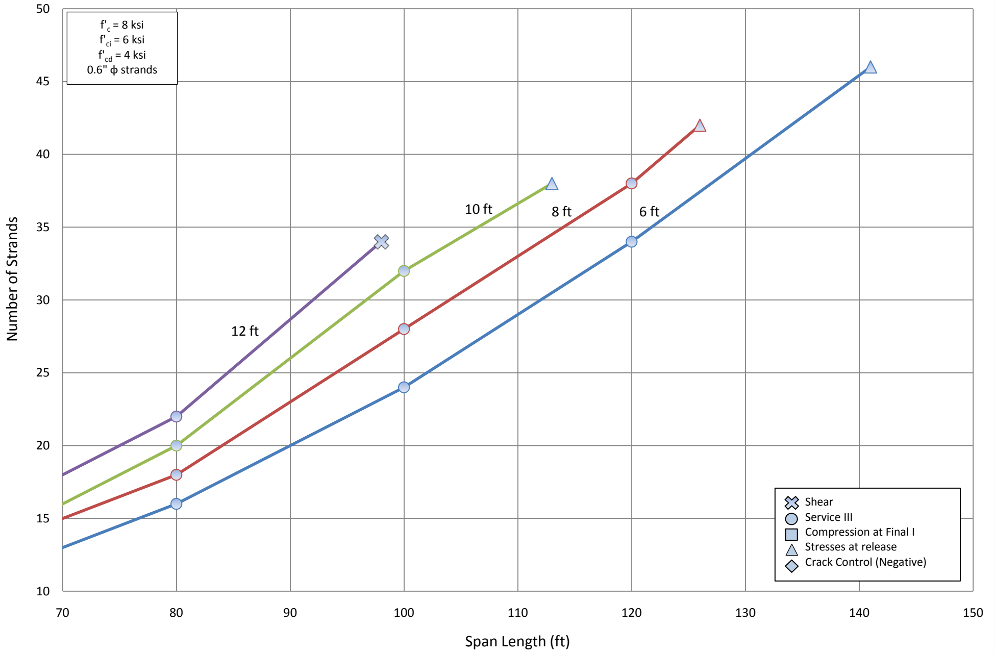
Number of Strands for NU 1100 - Two Span
