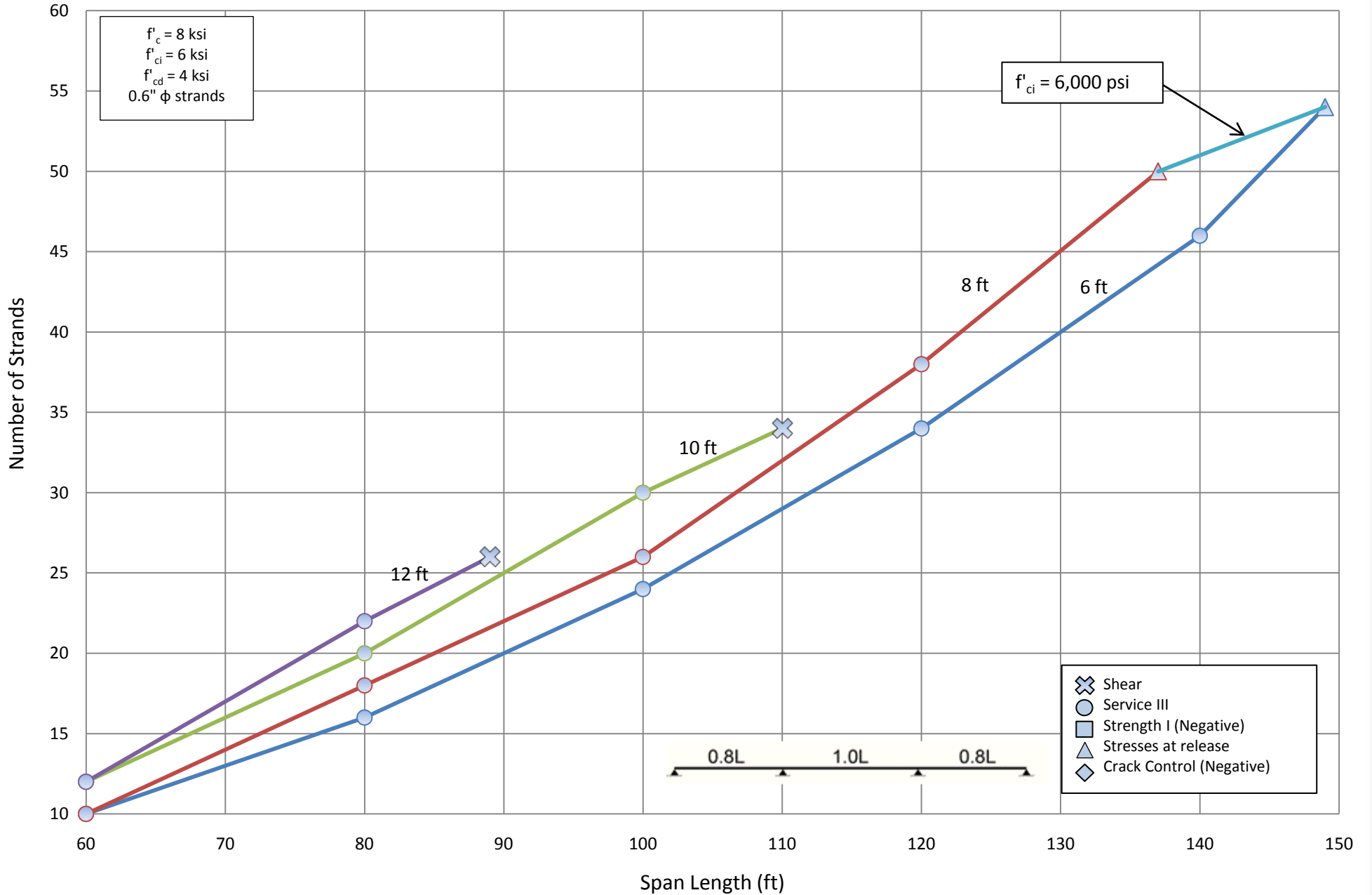
Number of Strands for NU 900 - Three Span (1.0L)
