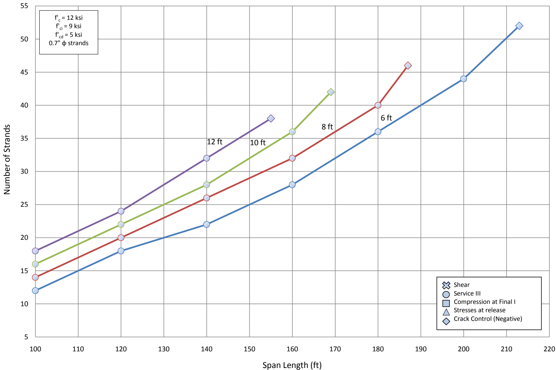
Number of Strands for NU 1600 - Two Span
