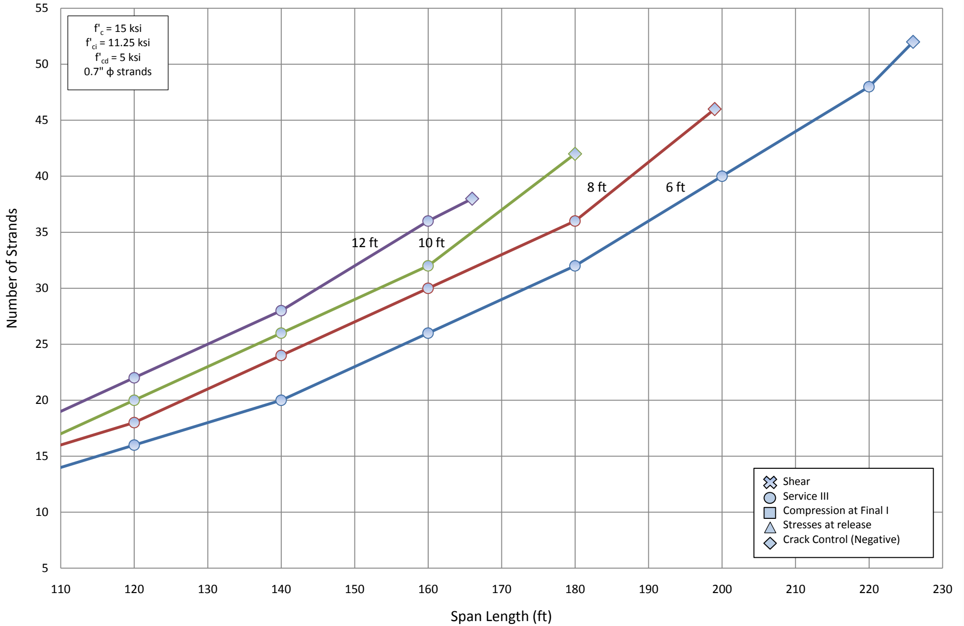
Number of Strands for NU 1800 - Two Span
