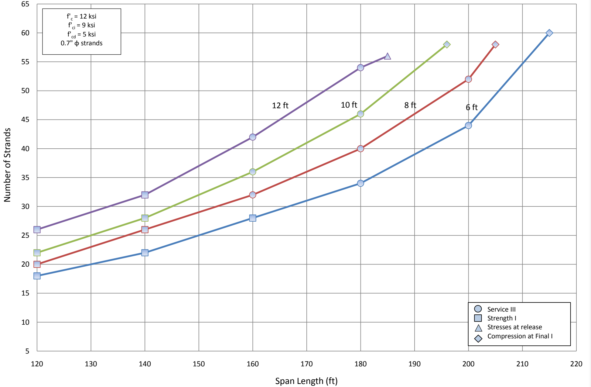
Number of Strands for NU 2000 - Simple Span
