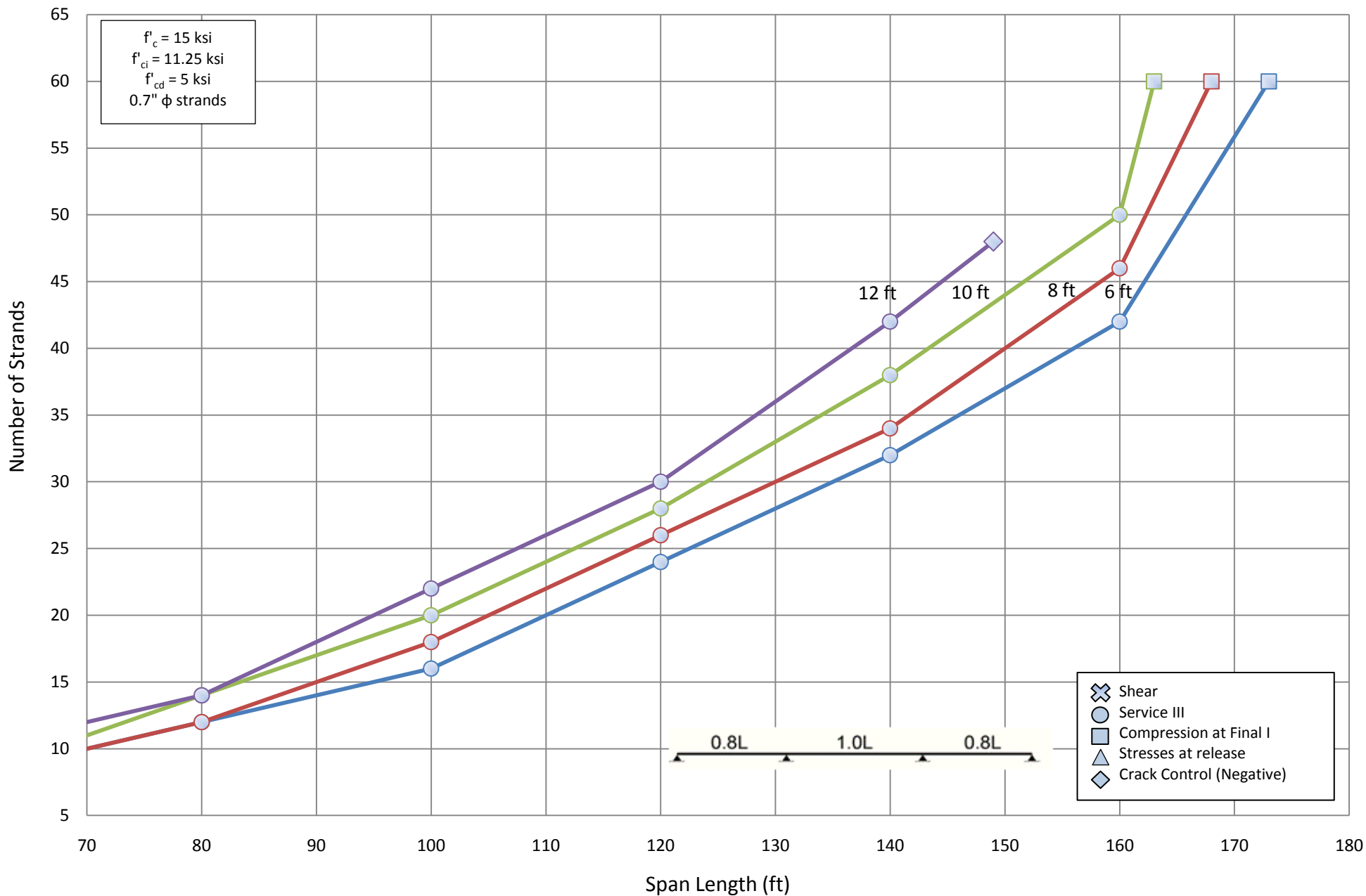
Number of Strands for NU 900 - Three Span (1.0L)
