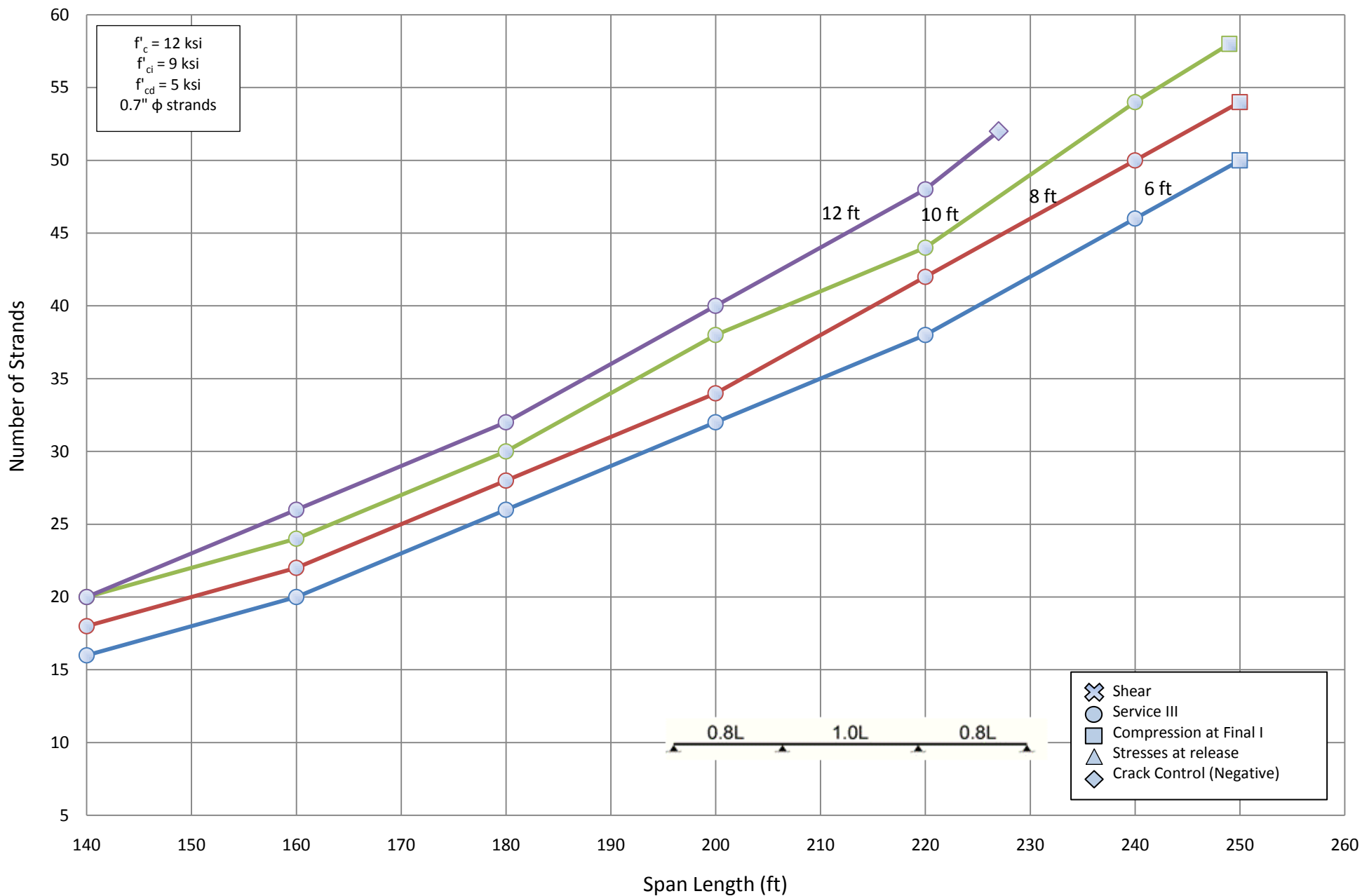
Number of Strands for NU 2000 - Three Span (1.0L)
