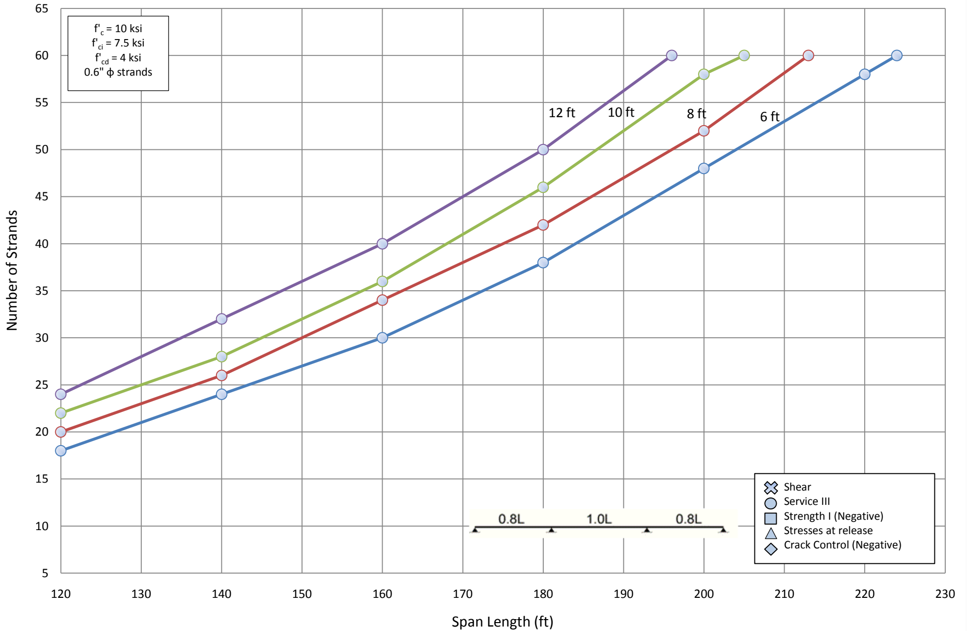
Number of Strands for NU 1800 - Three Span (1.0L)
