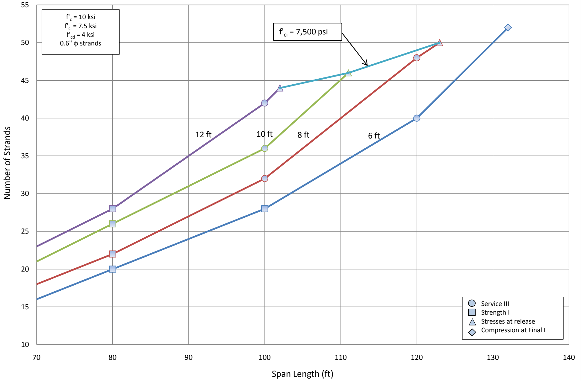
Number of Strands for NU 1100 - Simple Span
