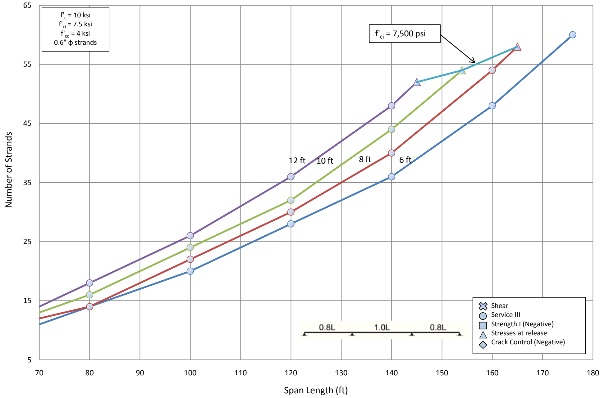
Number of Strands for NU 1100 - Three Span (1.0L)
