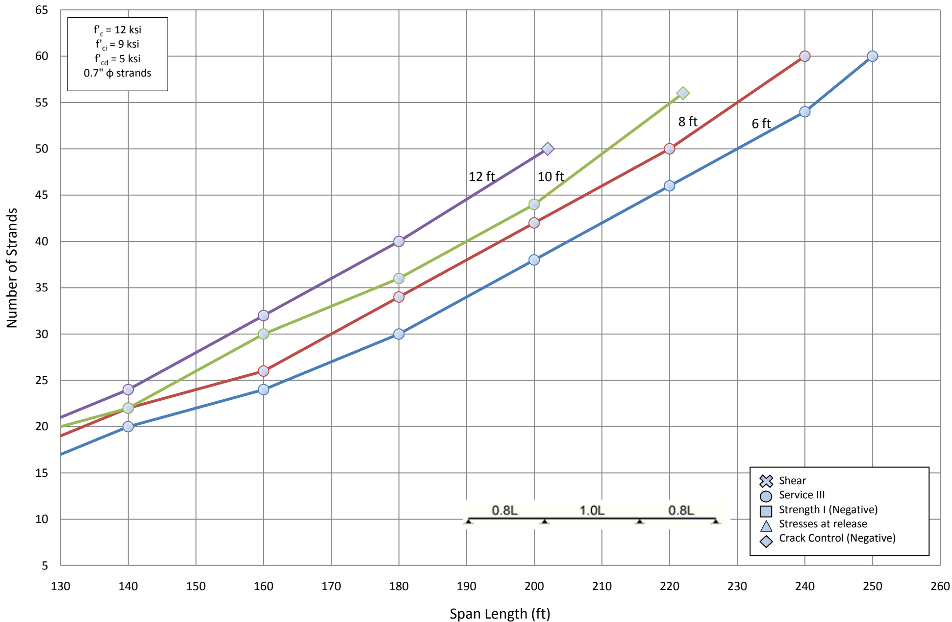
Number of Strands for NU 1600 - Three Span (1.0L)
