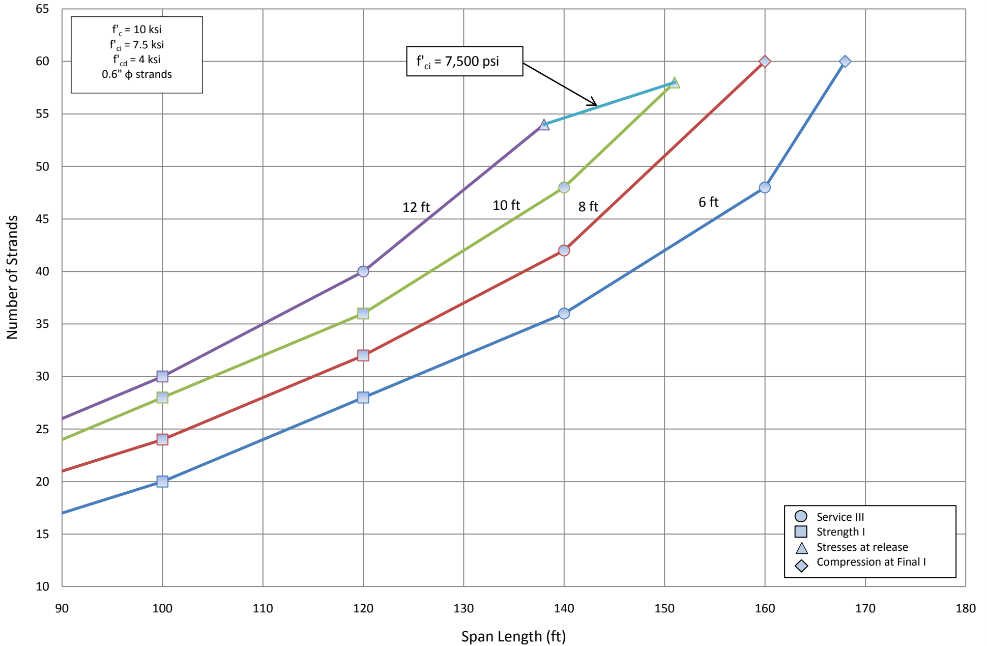
Number of Strands for NU 1600 - Simple Span
