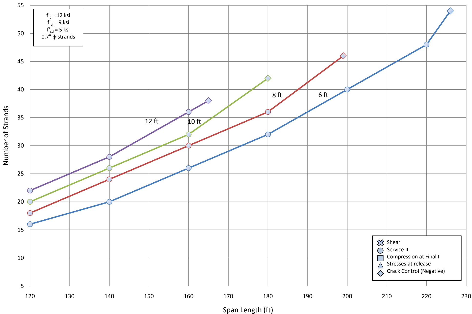
Number of Strands for NU 1800 - Two Span
