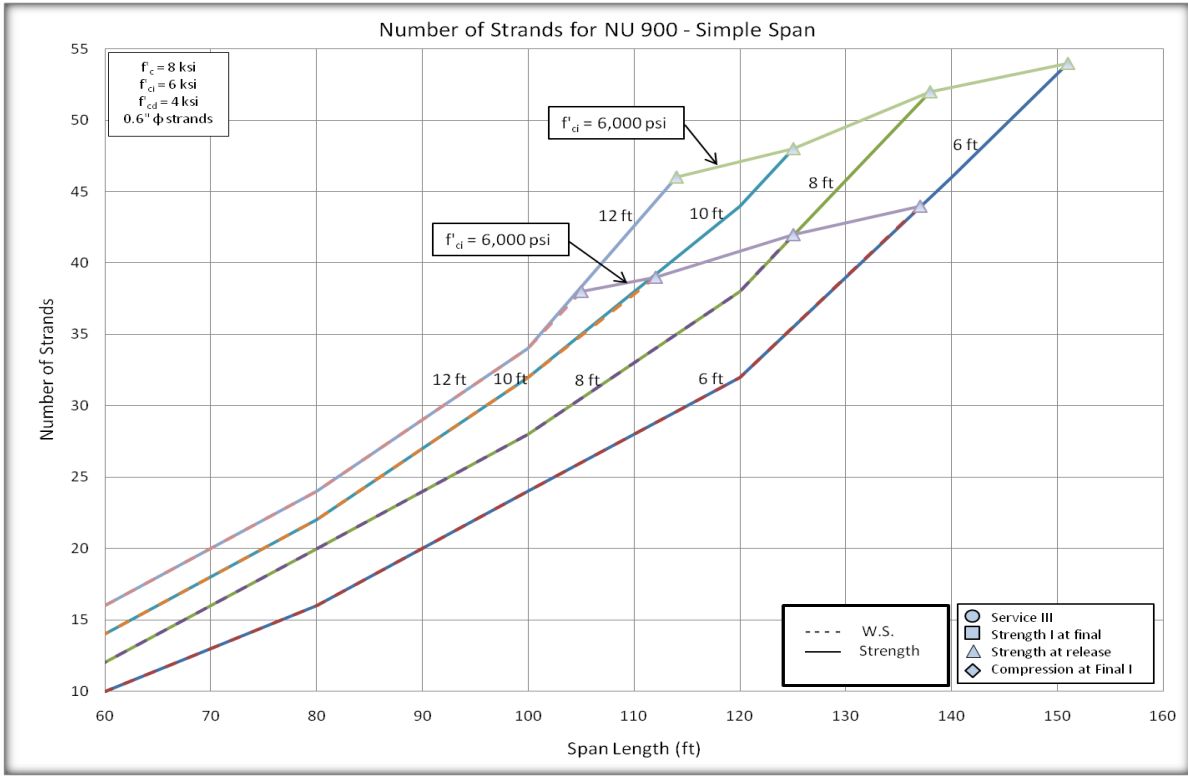
Figure 10 Detailed chart comparing Strength Design Method and Working Stress Method.
