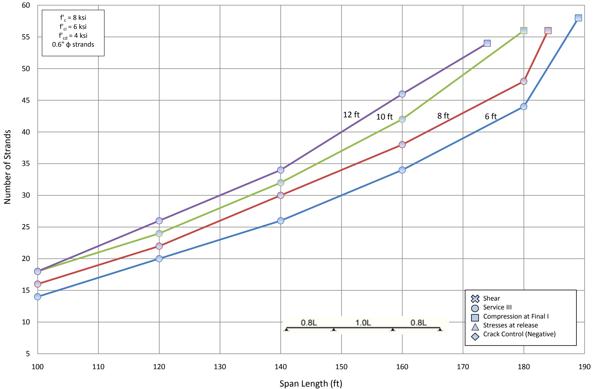
Number of Strands for NU 1600 - Three Span (1.0L)
