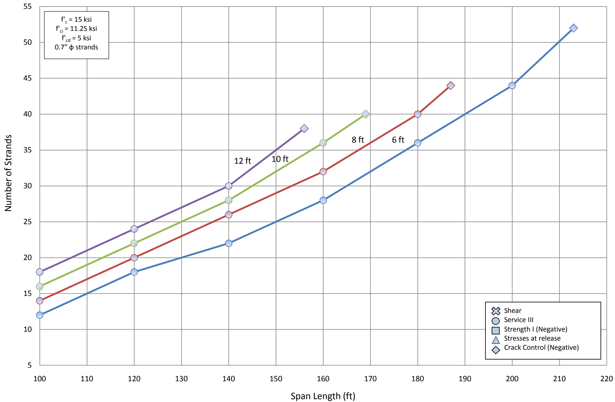
Number of Strands for NU 1600 - Two Span
