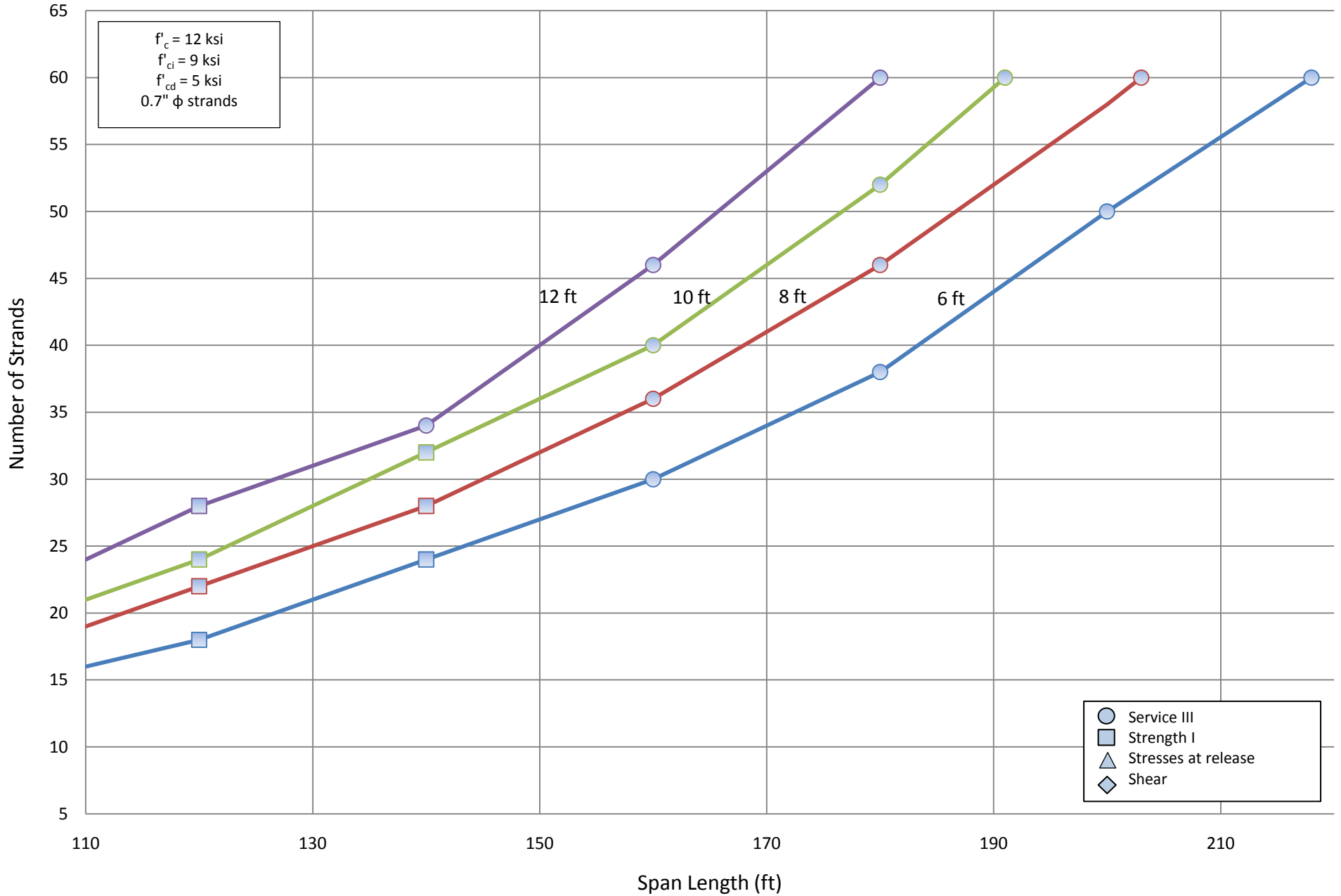
Number of Strands for NU 1800 - Simple Span
