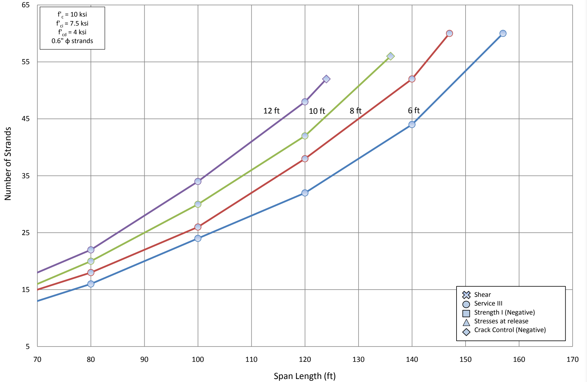
Number of Strands for NU 1100 - Two Span
