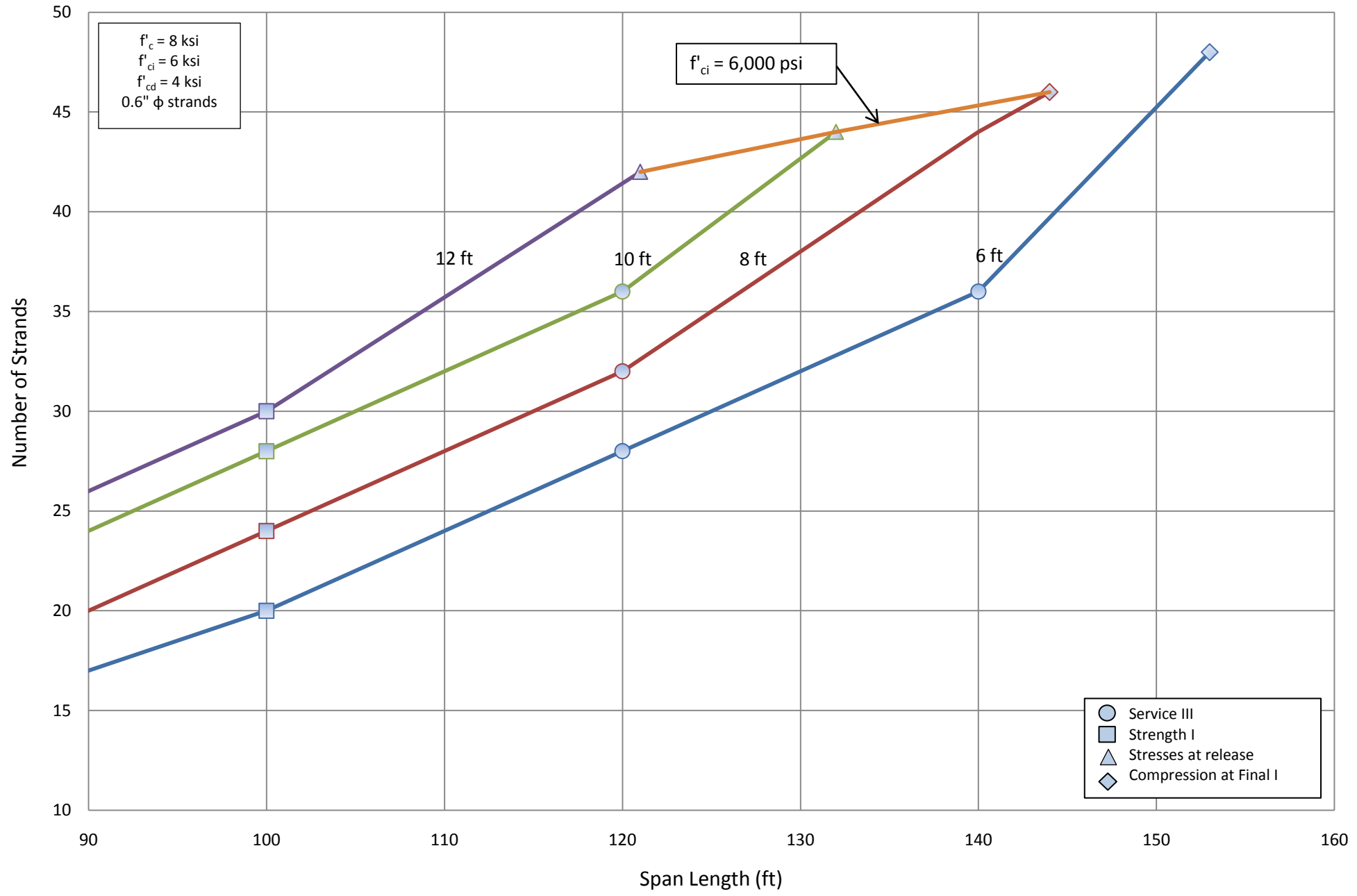
Number of Strands for NU 1600 - Simple Span
