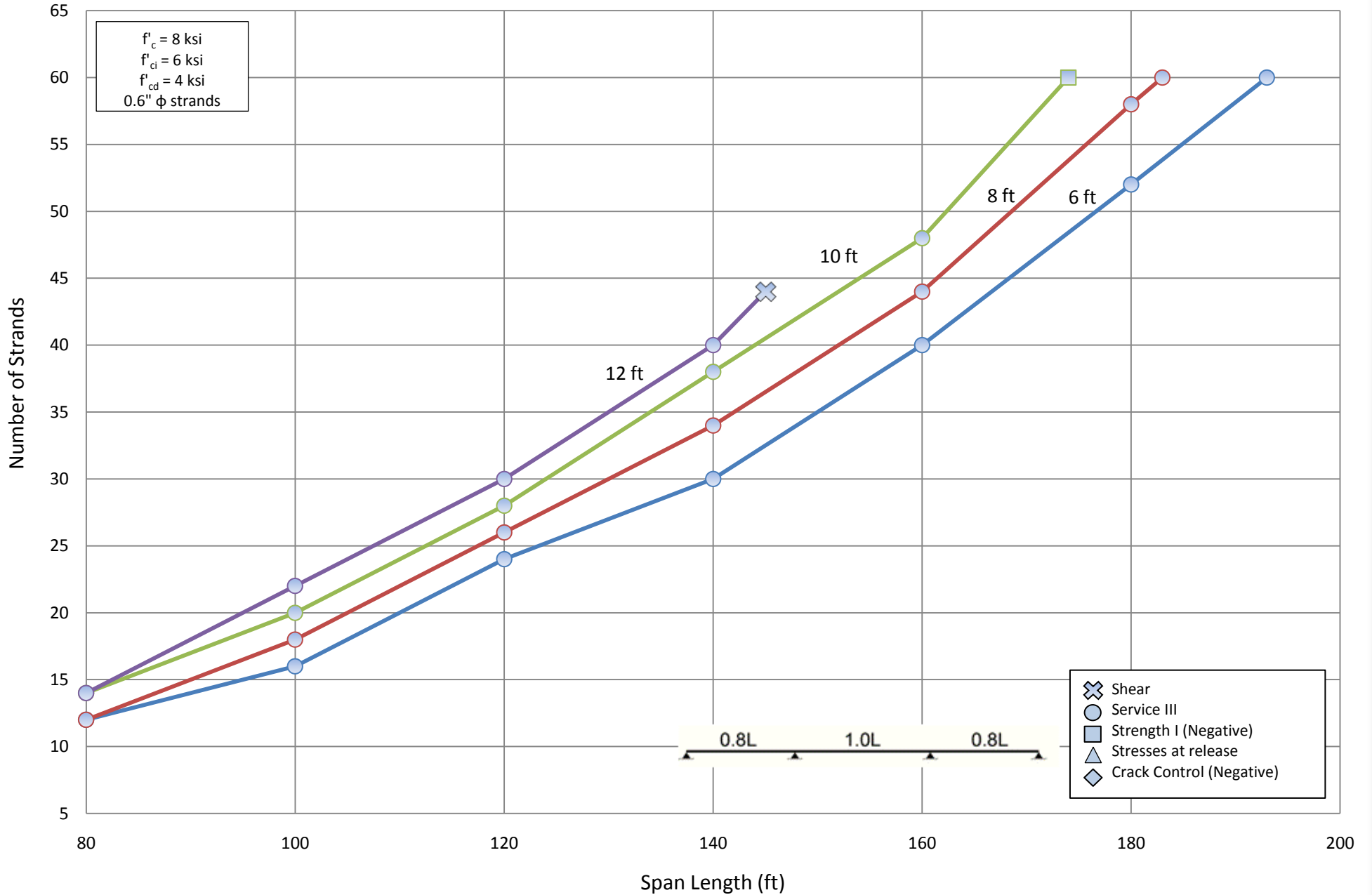
Number of Strands for NU 1350 - Three Span (1.0L)
