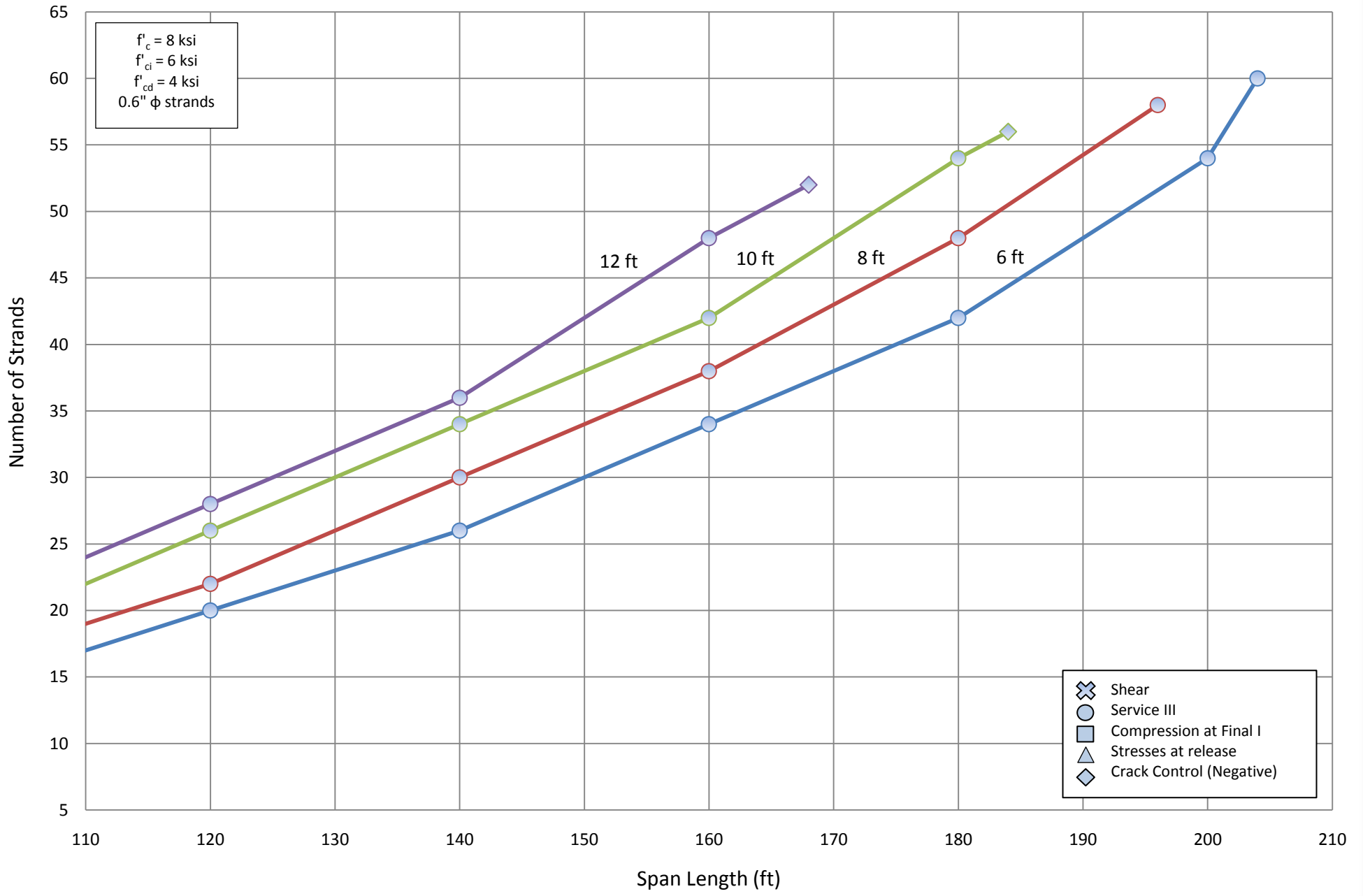
Number of Strands for NU 2000 - Two Span
