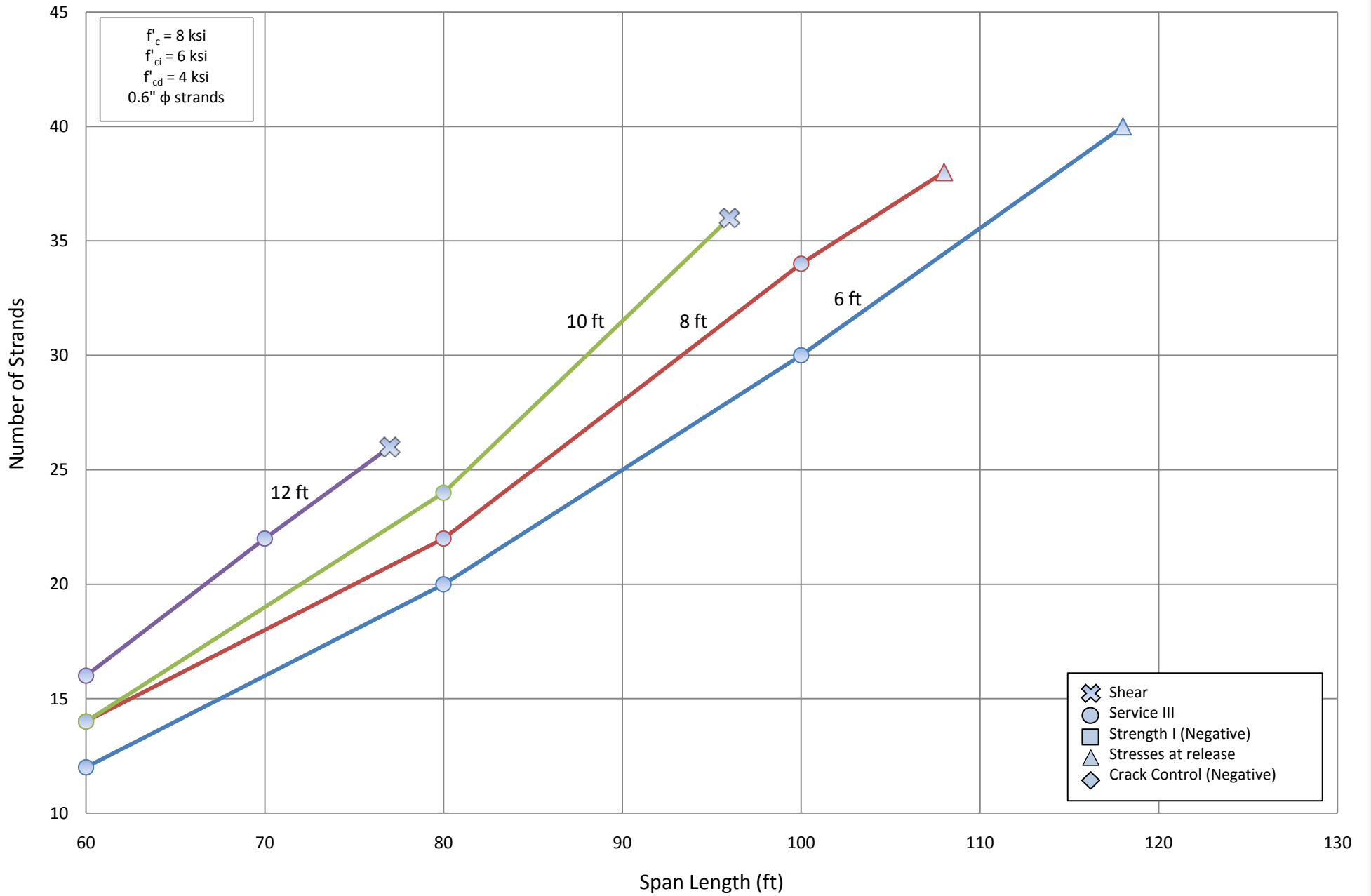
Number of Strands for NU 900 - Two Span
