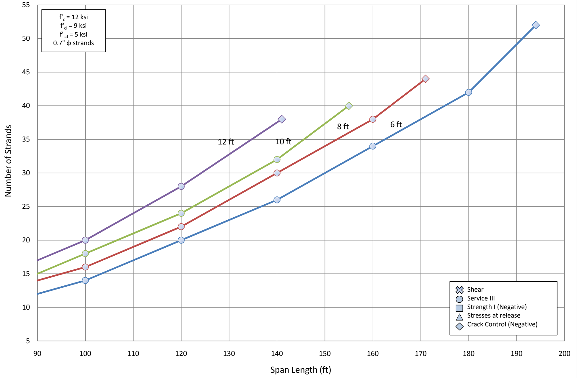
Number of Strands for NU 1350 - Two Span
