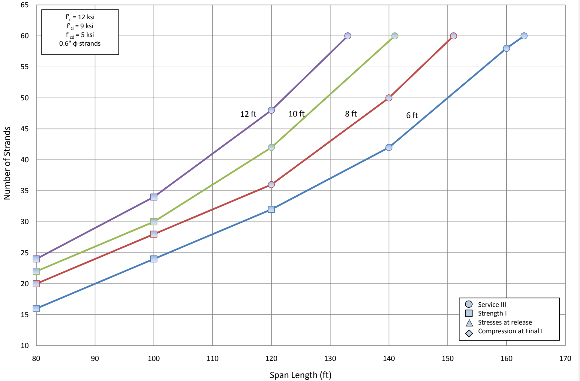
Number of Strands for NU 1350 - Simple Span
