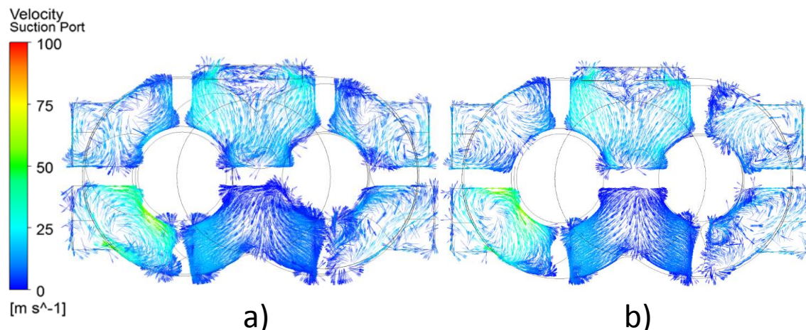
Figure 8 Velocity vector plot at the suction a) Full case b) Simplified model
