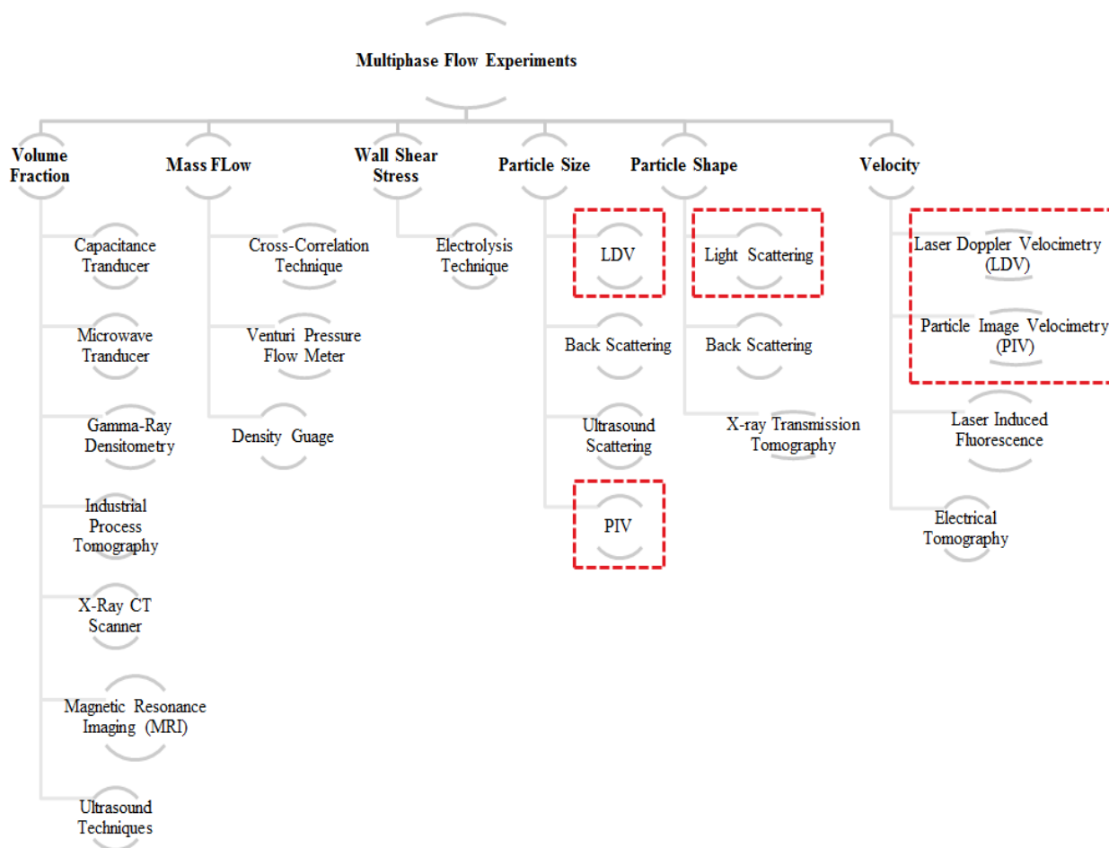
Figure 2 Experimental techniques in measuring multiphase flow parameters during the experiments
