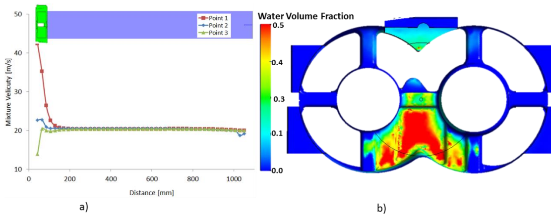
Figure 10 a) Mixture velocities through suction port b) Water depositions on the surface of the suction port
