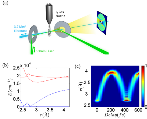
FIG. 1. (a) Diagram of the experimental setup showing the laser beam (green), electron beam (blue), and gas jet (gray). (b) Potential energy surfaces of ground state (dashed blue line) and the B excited state (dashed red line), along with the ground and excited state wave packets (solid lines). The blue and red colors represent ground and the excited states, respectively. (c) Simulated dynamics of the nuclear wave packet of I_2 in the B state, after excitation by a 530 nm laser pulse. The figure displays the amplitude of the wave function as a function of time, in arbitrary units.
