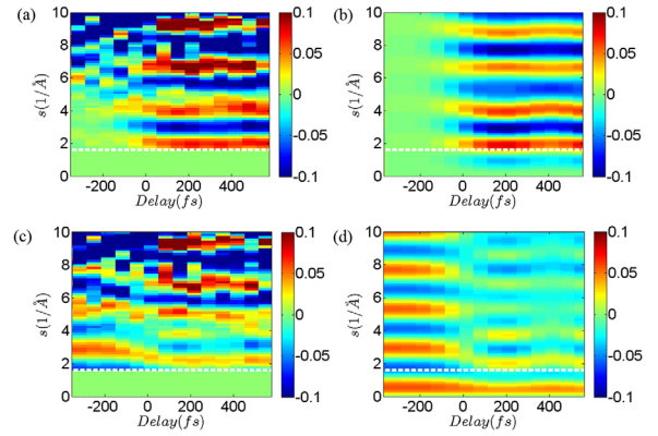
FIG. 3. (a),(b) The experimental (a) and simulated (b) time-resolved modified scattering intensity difference \Delta sM(t, s) . (c), (d) The experimental (c) and simulated (d) time-resolved modified scattering intensity of the excited state sM_{\text{Excited}}(t, s) . The pattern in (c) was generated by adding the known contribution from ground state to the experimental pattern in (a). The pattern in (d) was generated by adding the known contribution from ground state to the simulated pattern in (b). The experiment misses s values between 0 and 1.6 \text{ \AA}^{-1} (area underneath the white dashed line in each pattern) due to a hole in the detector that serves to transmit the main electron beam.
