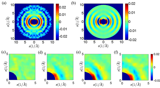
FIG. 2. (a) Experimental difference diffraction pattern \langle \Delta I_{\text{exp}}(t, s, \phi) \rangle averaged over t = 50 fs to 550 fs. (b) Simulated difference diffraction pattern \langle \Delta I_{\text{sim}}(t, s, \phi) \rangle averaged over t = 50 fs to 550 fs. The color scales are in arbitrary units. (c) through (f): experimental difference diffraction patterns \Delta I_{\text{exp}}(ts, \phi) at t = -184 fs, t = 17 fs, t = 217 fs, and t = 417 fs, respectively.
