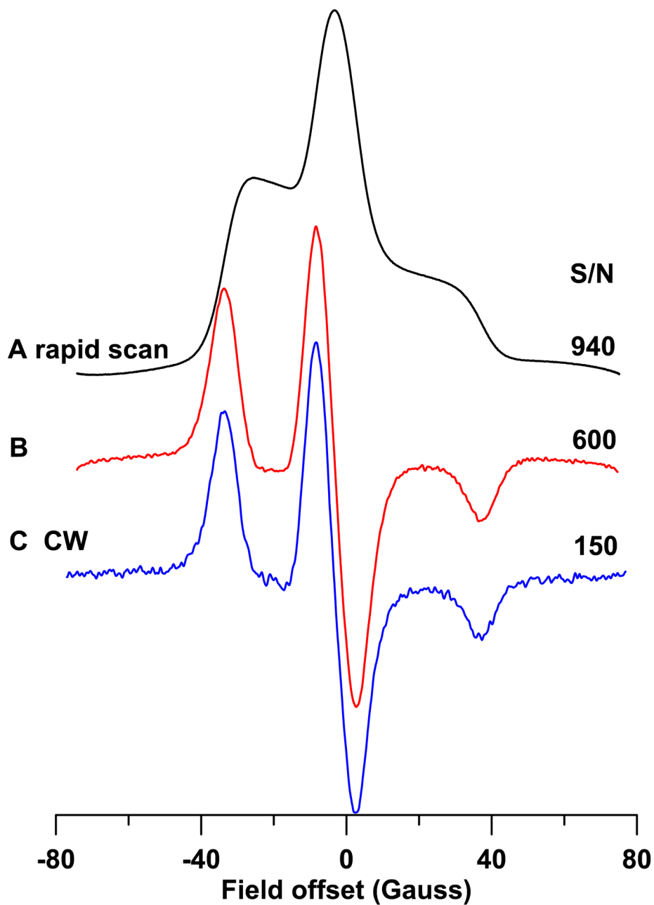
Figure 4. CW and rapid-scan spectra at 293 K of spin label 2 attached to T4 lysozyme obtained with 10 s acquisition times. (A) Absorption spectrum obtained by rapid-scan with the parameters listed in Table 2, (B) first derivative obtained from (A) by numerical differentiation, (C) field-modulated CW spectrum obtained with 100 kHz modulation frequency and 1.8 G modulation amplitude which is 20% of B_{pp} = 1.06 G
