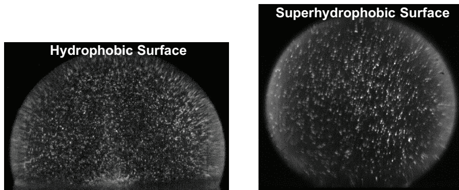
Center-plane illuminated by laser light sheet
