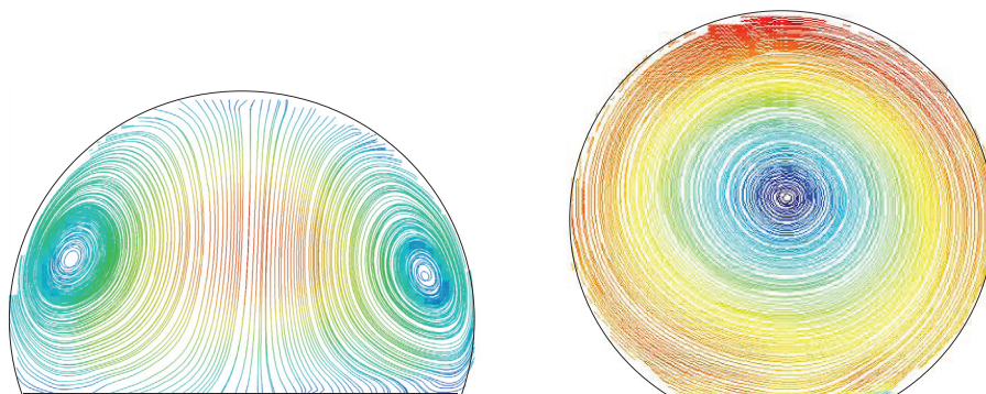
Representative streamlines
