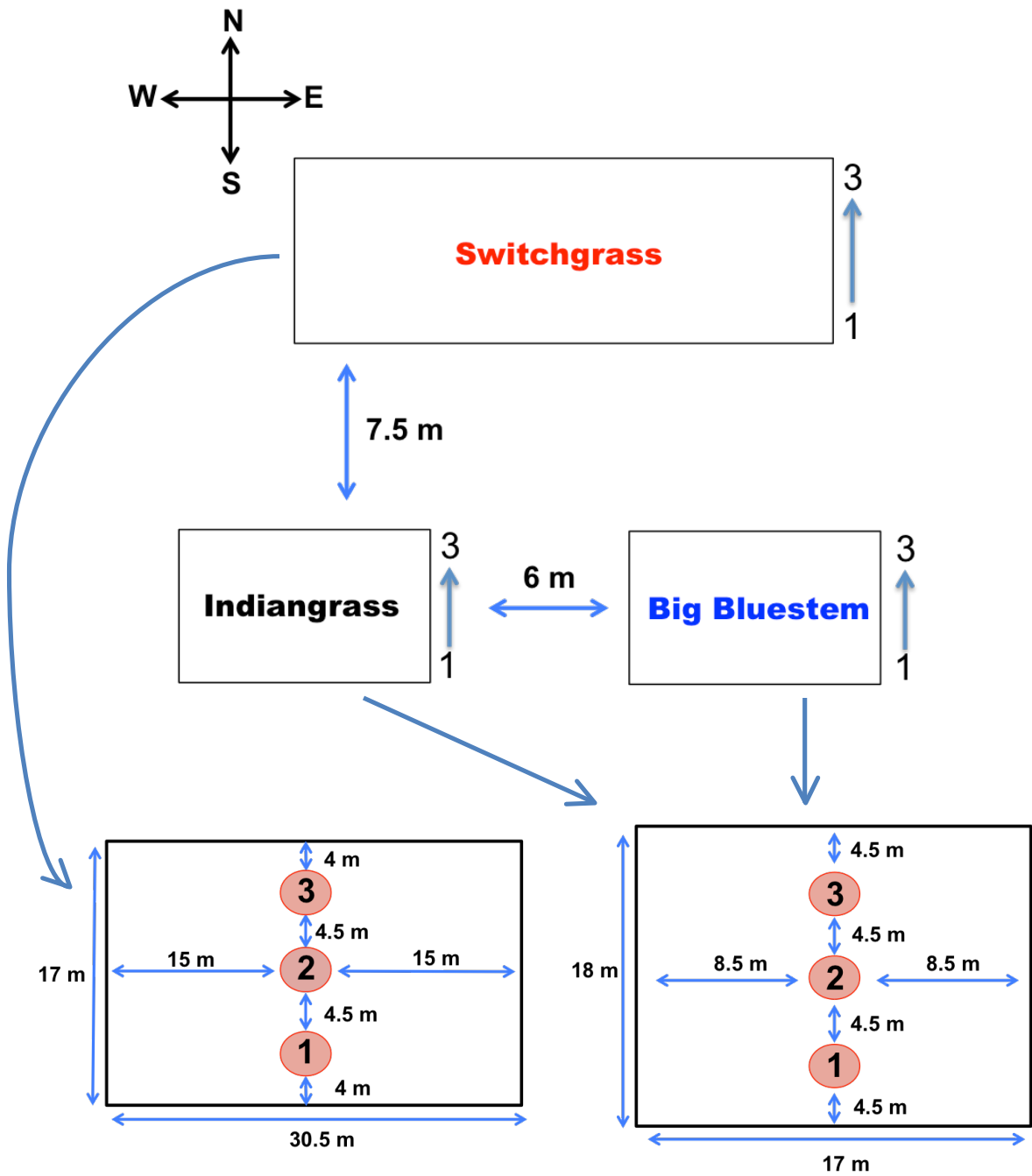
Figure 2.2 – Design layout for Study 2
