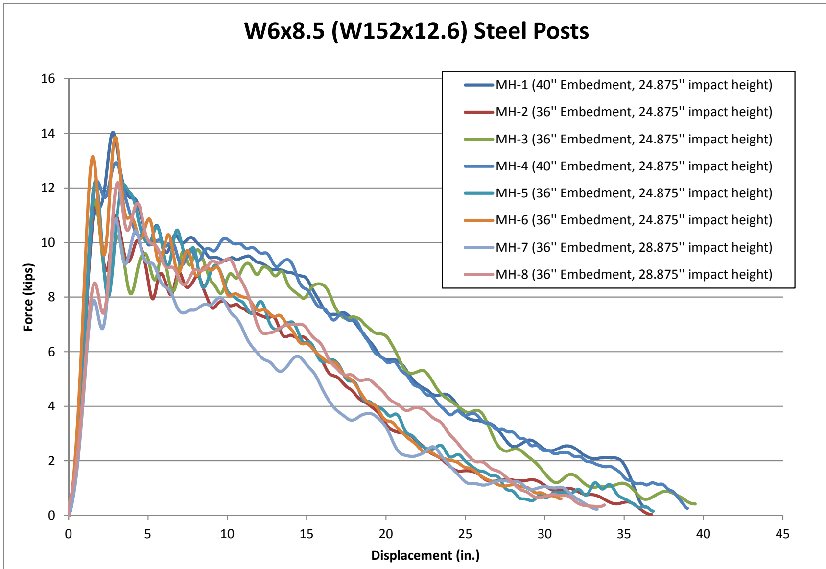
Figure 20. Force vs. Deflection Comparison, Test Nos. MH-1 through MH-8
