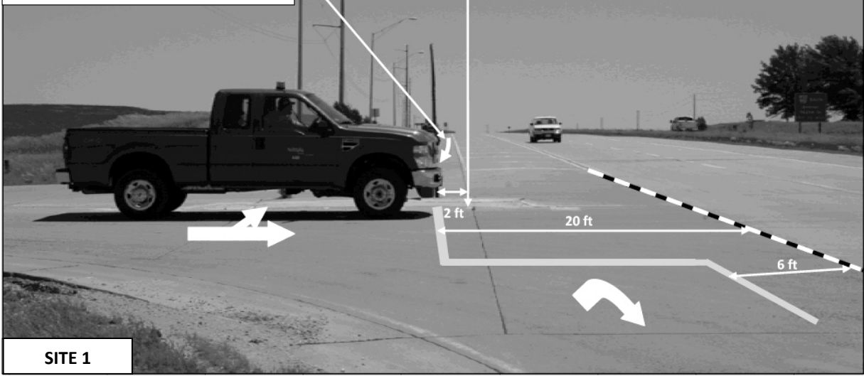
FIGURE 63 Improvements of Visual Cues at Site 1
