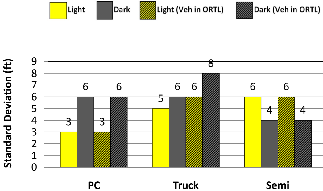
FIGURE 20 Standard Deviation of Vehicle Bumper Position from Near Edge of Major Road Through Lane by Vehicle Type at SB Stop-Controlled Approach, Site 1
