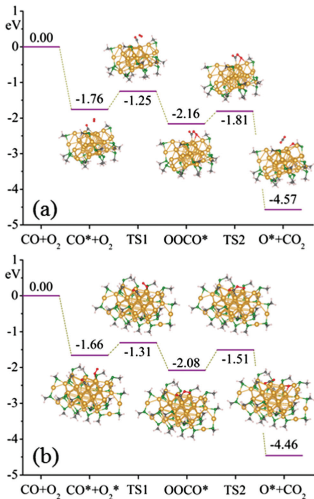
Fig. 6 Computed reaction pathway for the CO oxidation on Au 40 (SR) 24 (a) and Au 52 (SR) 32 (b) clusters. Here, the symbol * denotes adsorption of the corresponding molecules on Au atoms. Au, S, C, O, and H atoms are in gold, olive, dark gray, red, and white, respectively.
