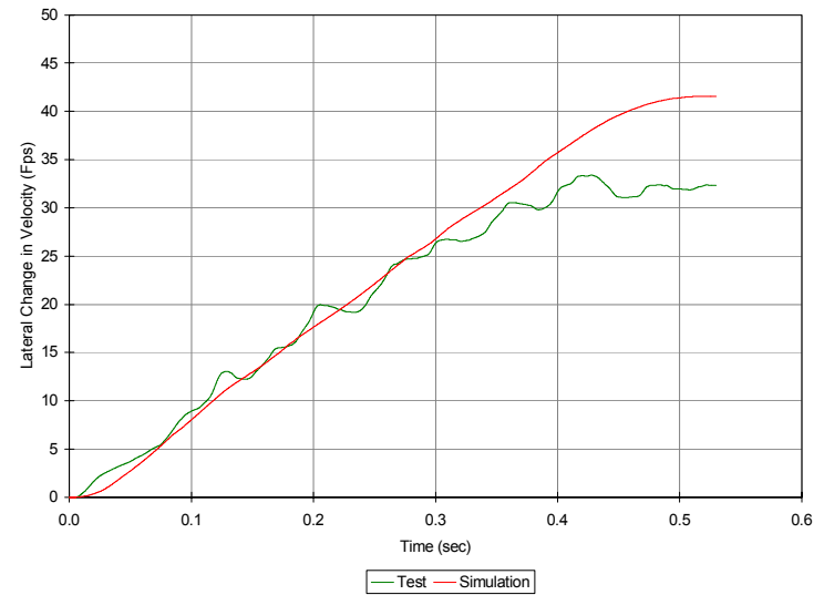
Figure 147. Comparison of Test and Simulation Results for Test NPG-4: (a) Longitudinal Direction and (b) Lateral Direction
