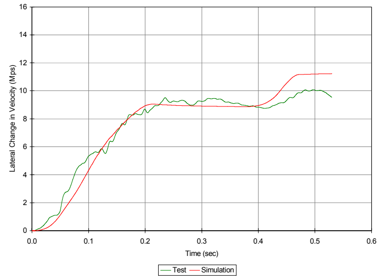
Figure 148. Comparison of Test and Simulation Results for Test NPG-6: (a) Longitudinal Direction and (b) Lateral Direction
