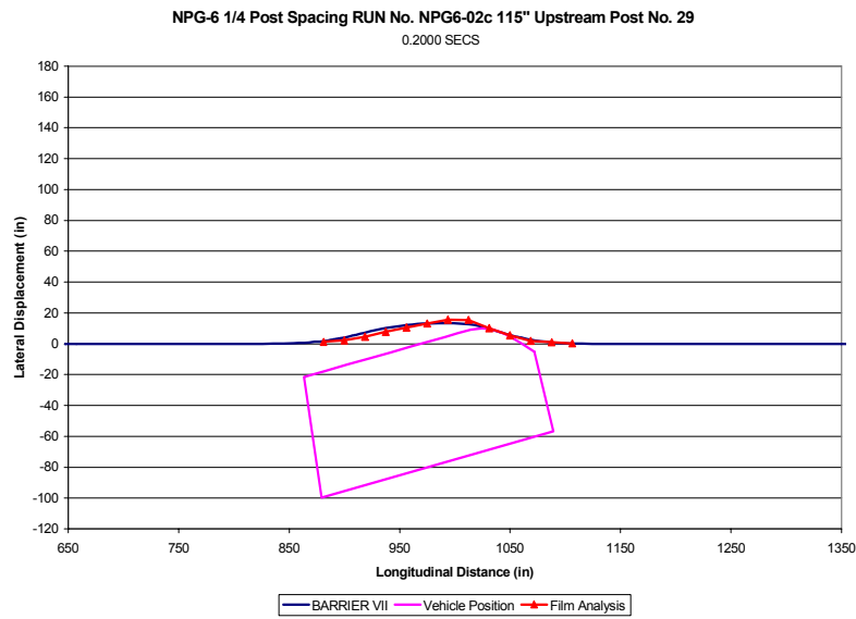
Figure 141. Sequential Figures from BARRIER VII Simulation of NPG-6
