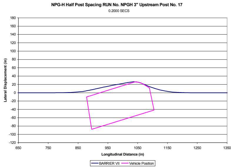
Figure 144. Sequential Figures from BARRIER VII Simulation of NPG-H
