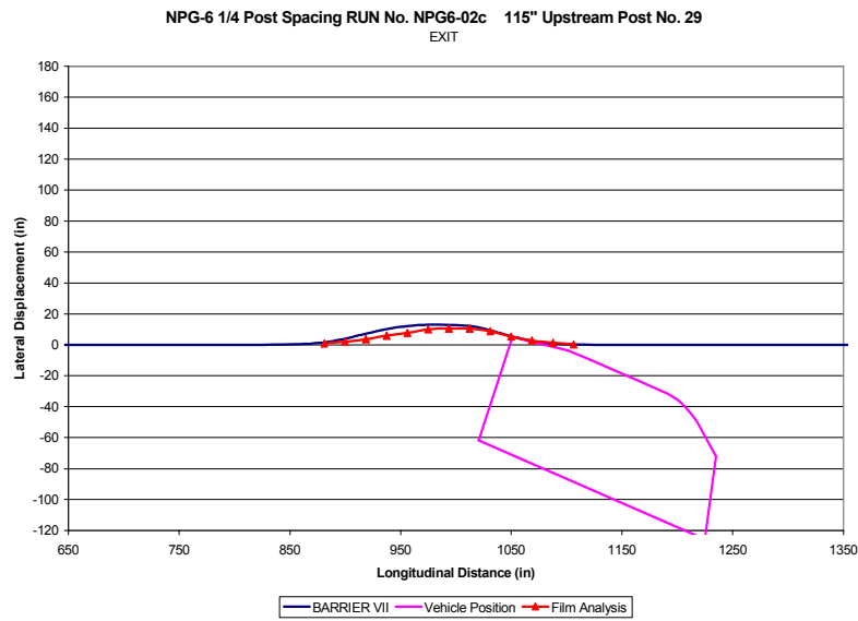
Figure 142. Sequential Figures from BARRIER VII Simulation of NPG-6 (continued)
