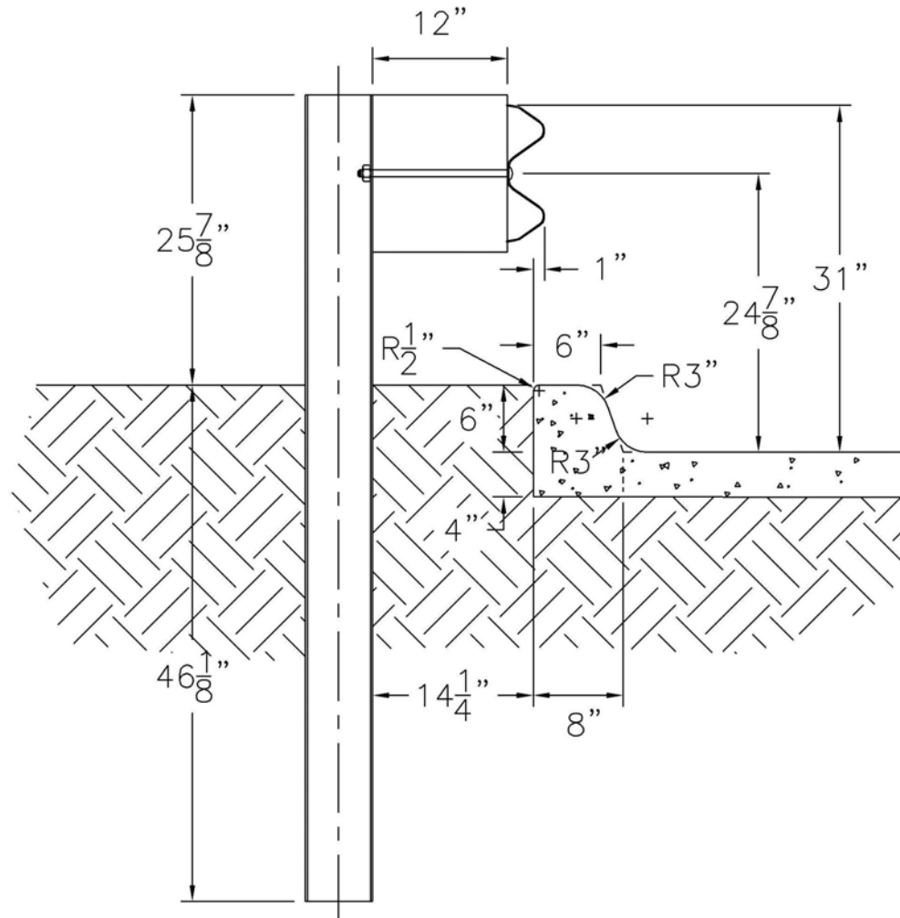
Figure H-9. Midwest Guardrail System Standard Post Spacing with Curb - System Profile (English)
