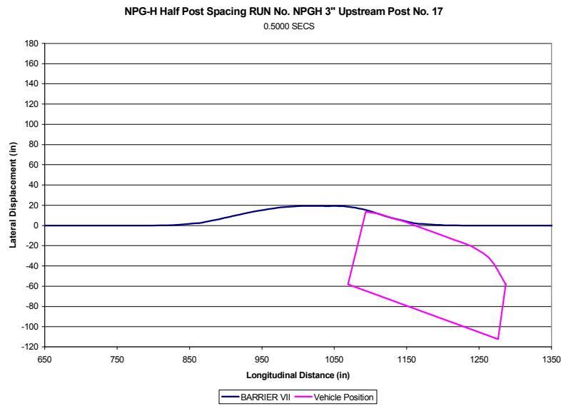
Figure 145. Sequential Figures from BARRIER VII Simulation of NPG-H (continued)
