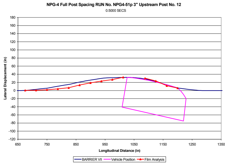
Figure 139. Sequential Figures from BARRIER VII Simulation of NPG-4 (continued)
