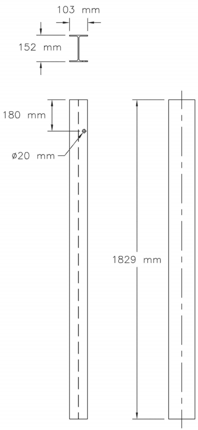
Figure J-5. Midwest Guardrail System Reduced Post Spacing - Post Design Details (Metric)
