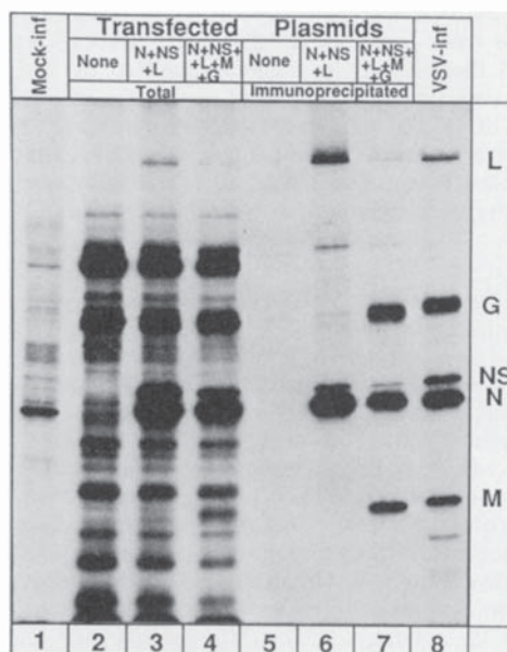
FIG. 1. Coexpression of VSV proteins in cotransfected cells. Cells infected with vTF7-3 and transfected with no plasmid (lanes 2 and 5), 5 \mu g of pAP-L, 10 \mu g of pMB-NS, and 15 \mu g of pAP-N (lanes 3 and 6), or 5 \mu g of pAP-L, 10 \mu g of pMB-NS, 15 \mu g of pAP-N, 10 \mu g of pKOM2, and 15 \mu g of pTF-G (lanes 4 and 7) were labeled with [ 35 S]methionine. Total cytoplasmic proteins (lanes 2-4) or proteins immunoprecipitated from cytoplasmic extracts with anti-VSV antibodies (lanes 5-7) were analyzed by SDS/PAGE. Proteins from mock-infected (lane 1) and VSV-infected (lane 8) cells are also shown.
