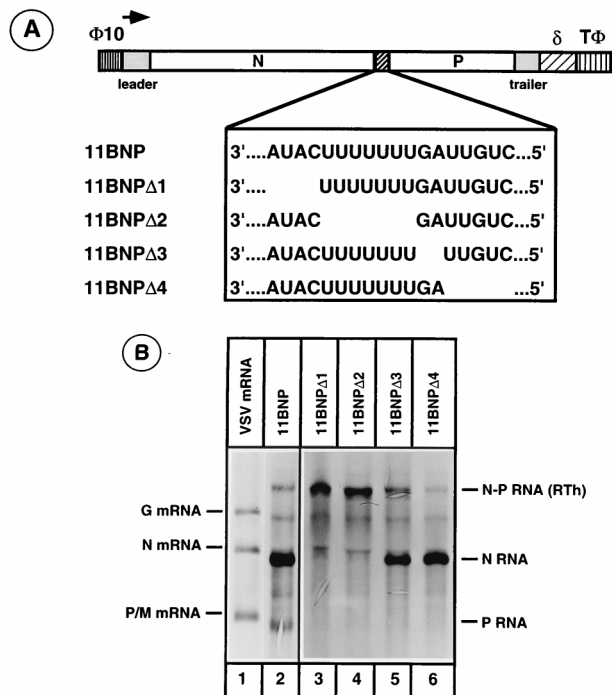
FIG. 3. (A) 11BNP and mutant minireplicons encoding deletion of various regions of the intercistronic gene junction. (B) Analysis of RNAs generated from various deletion mutant minireplicons. Cells were infected with vTF7-3 and cotransfected with plasmids encoding the minireplicons as well as the N, P, and L proteins. Cells were labeled with [ ^3 H]uridine and [ ^3 H]adenosine in the presence of actinomycin D and AraC as described in Materials and Methods. Total labeled RNAs from cytoplasmic extracts of cells were electrophoresed in an acid-agarose urea gel and detected by fluorography. Lane 1 shows VSV mRNAs from infected cells. VSV RNA polymerase catalyzed transcription products are shown on the right. RTh, readthrough product of transcription.
