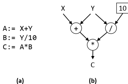
Figure 2.4: An example of a simple program (a) and its dataflow equivalent (b), shown as proposed by Johnston et al. [17].
