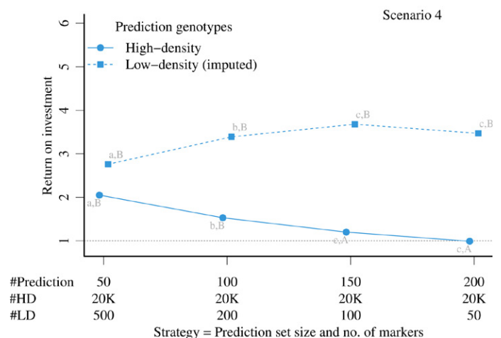
Fig. 5. Return on investment for selection within a family against the number of selection candidates having the true high-density genotypes (HD) or low-density genotypes imputed to high density (LD); 2000 training individuals had the true high-density genotypes (letters denote significant difference between strategies [the first letter] and the baseline scenario [the second letter] at p \leq 0.01 according to the Tukey's multiple comparison test).
