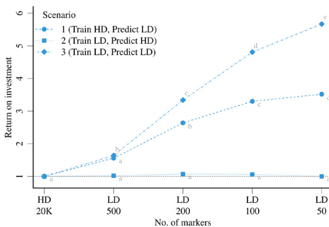
Fig. 3. Return on investment for selection within a family against the number of markers used in the training set with 2000 individuals and prediction set with 200 individuals; HD, true high-density genotypes; LD, low-density genotypes imputed to high density; letters denote significant difference within a scenario at p \leq 0.01 according to the Tukey's multiple comparison test.
