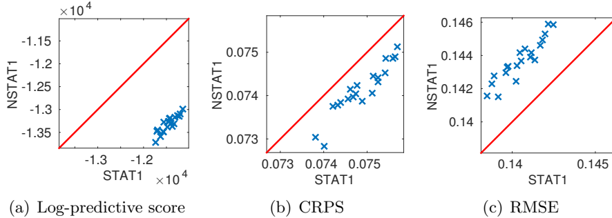
Figure 13: Scatter plots of (a) Log-predictive score, (b) CRPS and (c) Root mean square error for STAT1 and NSTAT1. The estimates were calculated with hold-out sets where 20% of the locations were held-out from each year as described in Section 4.3.
