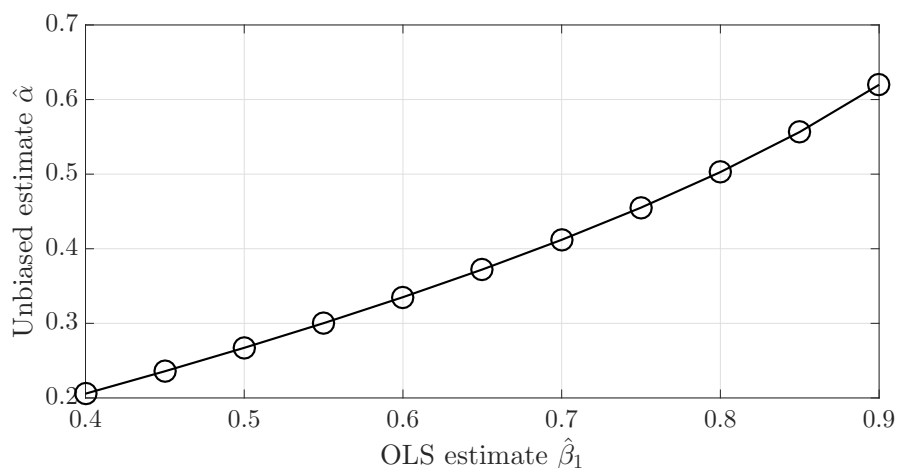
Figure D1: Relationship between biased and unbiased estimates of the matching function elasticity of hires with respect to vacancies ( \alpha )
