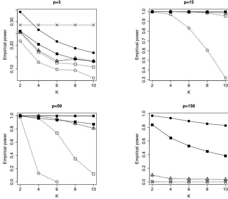
Figure 1: Plots of empirical power against lag K for the new tests T_n (solid and ■ lines) and T_n^* (solid and ● lines), the portmanteau tests Q_1 (dashed and \Delta lines), Q_2 (dashed and + lines) and Q_3 (dashed and □ lines), the Lagrange multiplier test (dashed and o lines), and Tiao and Box' test (dashed and \times ). The data are generated from Model 4 with sample size n = 300 . The nominal level is \alpha = 5\% .
