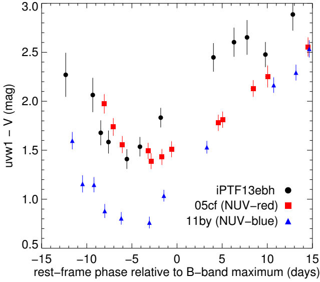
Fig. 6. u_w1 - V color curves of iPTF13ebh, SNe 2005cf, and 2011by. SNe 2005cf and 2011by are examples of the NUV-red and NUV-blue groups, respectively. The u_w1 - V color of iPTF13ebh is similar to that of the NUV-red group, but evolves faster.
