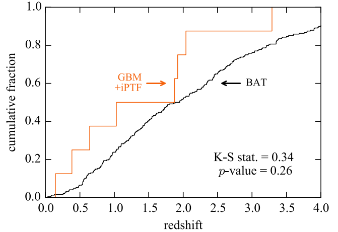
Figure 7. Cumulative distribution of redshifts of long GRBs observed by Swift BAT (gray) and the GBM–iPTF experiment (orange).
