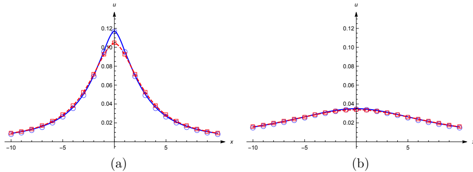
FIGURE 6.6. The solutions of (6.1), (6.2) for L = \tilde{L}_{M,s} (blue solid line with circles) and for L = cL_1^\alpha (red dashed line with squares) for t = 1 (a) and t = 3 (b).
