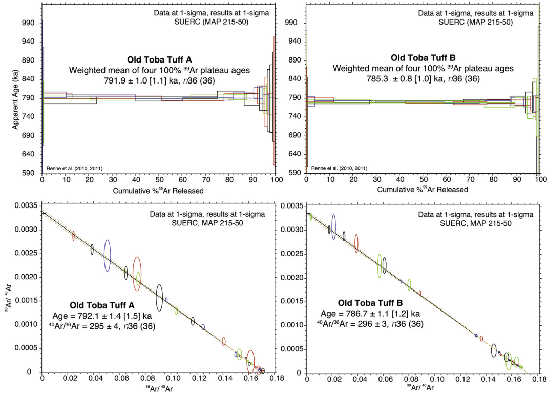
Fig. 6. Incremental step-heating 40 Ar/ 39 Ar age spectra and isotope correlation plots (OTTA and OTTB).
