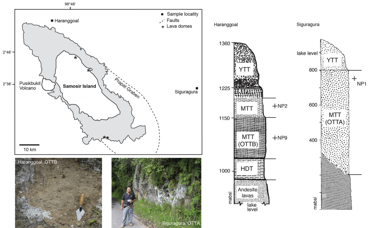
Fig. 3. Map showing the location of sampling sites relative to the Toba Caldera with the respective stratigraphies for both sites. Further details on the stratigraphic sequences are provided in the text.
