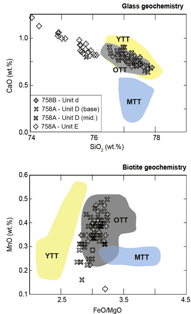
Fig. 4. Glass and biotite geochemistry for ODP 758 Ashes D, d and E as well as proximal YTT, MTT and OTT data from Siguragura and Harrangoal. Note the glass geochemistry cannot distinguish between the data from the YTT and OTT deposits, but the biotite shows a definitive correlation with the OTT. Ash E was distinctly lacking in biotite, only one crystal was found.
