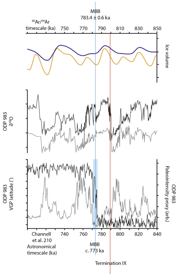
Fig. 14. Plot showing the record for both benthic (grey) and planktic (black) \delta^{18}\text{O} from ODP 983 (adapted from Channell et al., 2010 ). Also shown is Virtual Geomagnetic Polar (VGP) latitude (black) and relative intensity proxy (grey). Ice volume models based on midsummer (orange) and integrated summer (blue) insolation forcing are also plotted. The blue line shows the position of the MBB in the records and the blue box the duration of the MB-reversal at the site of ODP 983 as defined by the benthic \delta^{18}\text{O} . The lower x-axis shows the astronomical timescale as discussed by Channell et al. (2010) whereas the upper x-axis shows the revised chronology based on the high precision ^{40}\text{Ar}/^{39}\text{Ar} age constraints presented here. (For interpretation of the references to colour in this figure legend, the reader is referred to the web version of this article.)
