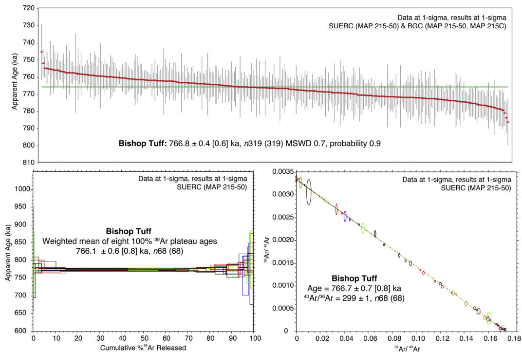
Fig. 7. 40 Ar/ 39 Ar single crystal fusion data and incremental step-heating age spectra and isotope correlation plots for Bishop Tuff sanidine.
