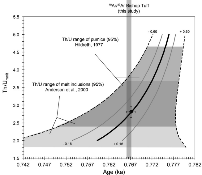
Fig. 10. Plot showing how the estimated \text{Th}/\text{U}_{\text{melt}} composition affects the ID-TIMS U–Pb zircon ‘eruption’ age (black circle) of Crowley et al. (2007) ( n17/19 ). The \text{Th}/\text{U}_{\text{melt}} is treated as a systematic variable, and so this uncertainty is propagated following determination of the weighted mean age. Uncertainty envelopes are shown for the \text{Th}/\text{U}_{\text{melt}} range ( \pm 0.16 ) used by Crowley et al. and what we consider to be a ‘more credible’ \text{Th}/\text{U}_{\text{melt}} range ( \pm 0.60 ) that reflects c. 68% of the variability seen in BT pumice and/or melt inclusions. Of note is the fact that the ^{40}\text{Ar}/^{39}\text{Ar} Bishop Tuff age reported in this study is consistent with the ID-TIMS U–Pb zircon age regardless of what \text{Th}/\text{U}_{\text{melt}} composition is assumed. Note all ages are shown including full external uncertainties and are displayed at the 2-sigma confidence level.
