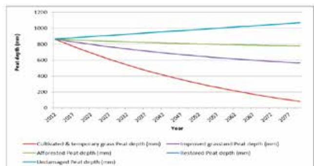
Box figure 1: Peat depth change under different land use scenarios assuming no climate change (from: Graves and Morris 2013).
